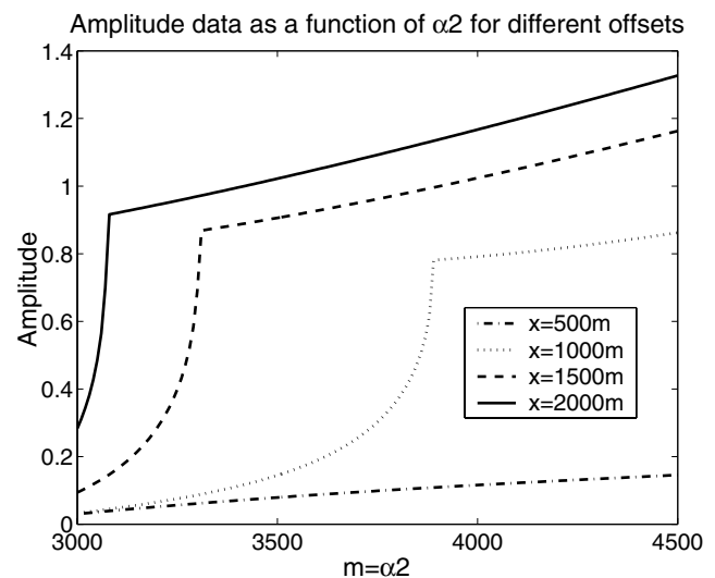
Figure 15. Amplitude data as a function of the model parameter \alpha_2 for 4 different offsets, x = 500 m, x = 1000 m, x = 1500 m and x = 2000 m. The velocity of the top layer is 2750 m s ^{-1} and the depth of the reflector is 500 m. The functions are calculated using dx = 0.001 , dm = 100dx and 100\,000 samples T .
