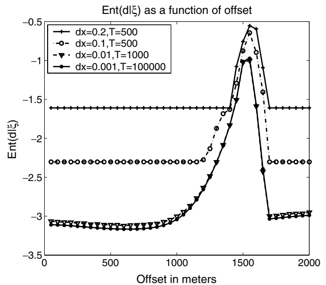
Figure 14. Ent(d|\xi) as a function of the offset in metres for the AVO example with a Gaussian uncertainty in the data space with a standard deviation of 0.01 . Velocity of the top layer is 2750 m s ^{-1} , the depth of the reflector is 500 m and the model parameter space runs from 3200 m s ^{-1} to 3300 m s ^{-1} . The entropy is calculated using four different discretizations and numbers of samples T . In all cases dm = 100dx has been used.
