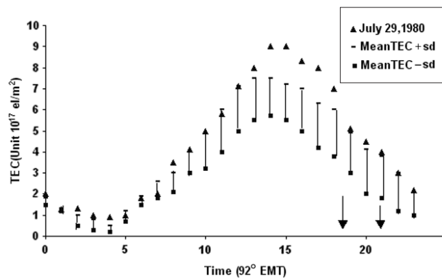
Fig. 4. Same as in fig. 3a,b but for high solar activity earthquake event. The event shown is for 29 July, 1980. Earthquake occurrence times are shown by arrowheads. The vertical bars give excursion of standard deviation of Q -day from the base.
