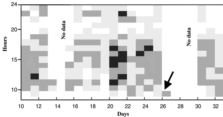
Fig. 8. A case of very strong earthquake of M = 8.1 experienced around Ahmedabad on 26 January, 2001. The large density contours followed by depletion in density prior to the event (at 09:00 h, 78°EMT) are clearly seen. Here the black region corresponds to frequencies > 11.50 MHz. Due to mass destruction no f_oF2 data are available just from the onset of the event for 3 days.
