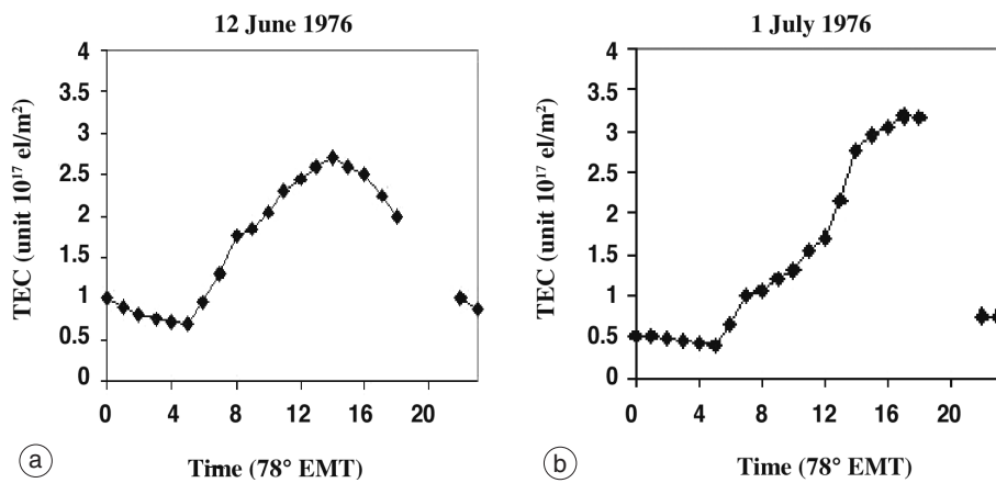
Fig. 1a,b. TEC variations during low solar activity period over Guwahati: a) a quiet day feature; b) a disturbed day TEC character. Note: the large enhancement in ionization density after sunset during the D -day.
