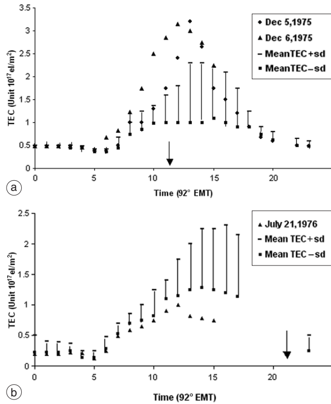
Fig. 3a,b. Plots showing variations in TEC (taken over Guwahati) from the Q -day base, during low solar activity period. Earthquakes occurred on (a) December 6, 1975 and (b) July 21, 1976. Earthquake commencement times are shown by arrowheads in the figure. The vertical bars give the excursion of standard deviation of Q -day TEC from the base.
