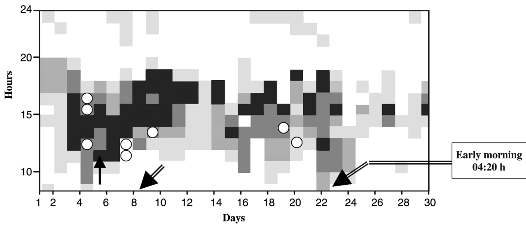
Fig. 7. Same as in figs. 5 and 6 but for three consecutive summer earthquake events for May 5, 8 and 22 of 1997. The arrowheads indicate the occurrence time of each earthquake event. Here the black zone is for frequencies > 10.00 MHz. White circles indicate absence of data. Though bite out is not prominent, high density zones up to day 23 are significant.
