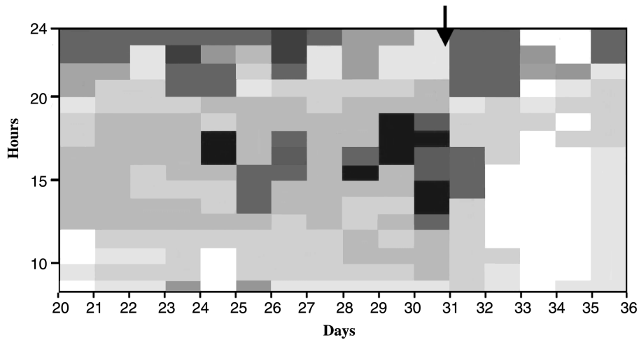
Fig. 6. One more case showing f_oF2 variations, prior to and during the 30.7.1996 earthquake. In this case the darkest region is for frequencies > 10.50 MHz. Presence of bite out is to be noted before the earthquake event.
