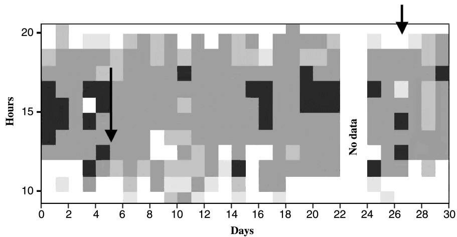
Fig. 5. f_oF2 variation pattern over the anomaly crest station of Ahmedabad before and during earthquakes of April 6 and 27, 1994. The arrowheads give the time of commencement of earthquakes. The density magnitude is defined by gray shades. Black zone is for frequencies > 11.00 MHz. Early morning data are not shown in the figure. High density zones and bite outs are present before and during the events.
