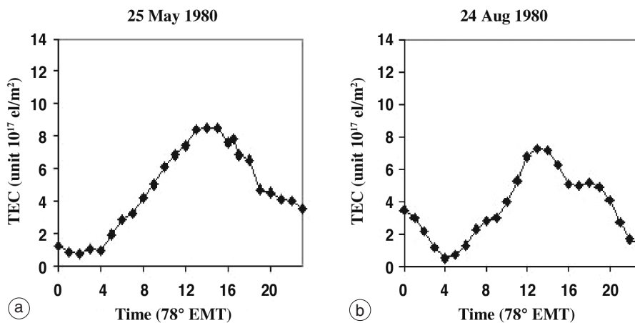
Fig. 2a,b. Same as in fig. 1a,b but for high solar activity periods: a) the usual quiet day diurnal variation and (b) one of the typical disturbed day TEC pattern. Note: the initial decay rate on D -day is arrested by post sunset enhancement.
