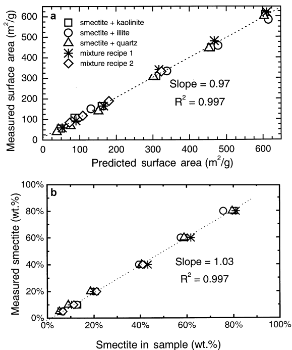
Figure 11. (a) The surface area measured by PVP uptake vs. the surface area predicted from the composition of the sample and the independently determined surface areas of the components. (b) The composition of the smectite measured in the samples by PVP uptake as a function of the amount of smectite mass added to the sample. The first three mixtures are variable amounts of smectite with the remaining portion of the sample containing a single additional phase. Recipe 1 is variable amounts of smectite with the remainder divided equally between kaolinite and illite. Recipe 2 is smectite plus 20% each of kaolinite and illite with the remainder quartz, except 80% smectite, which has 10% each of kaolinite and illite.
