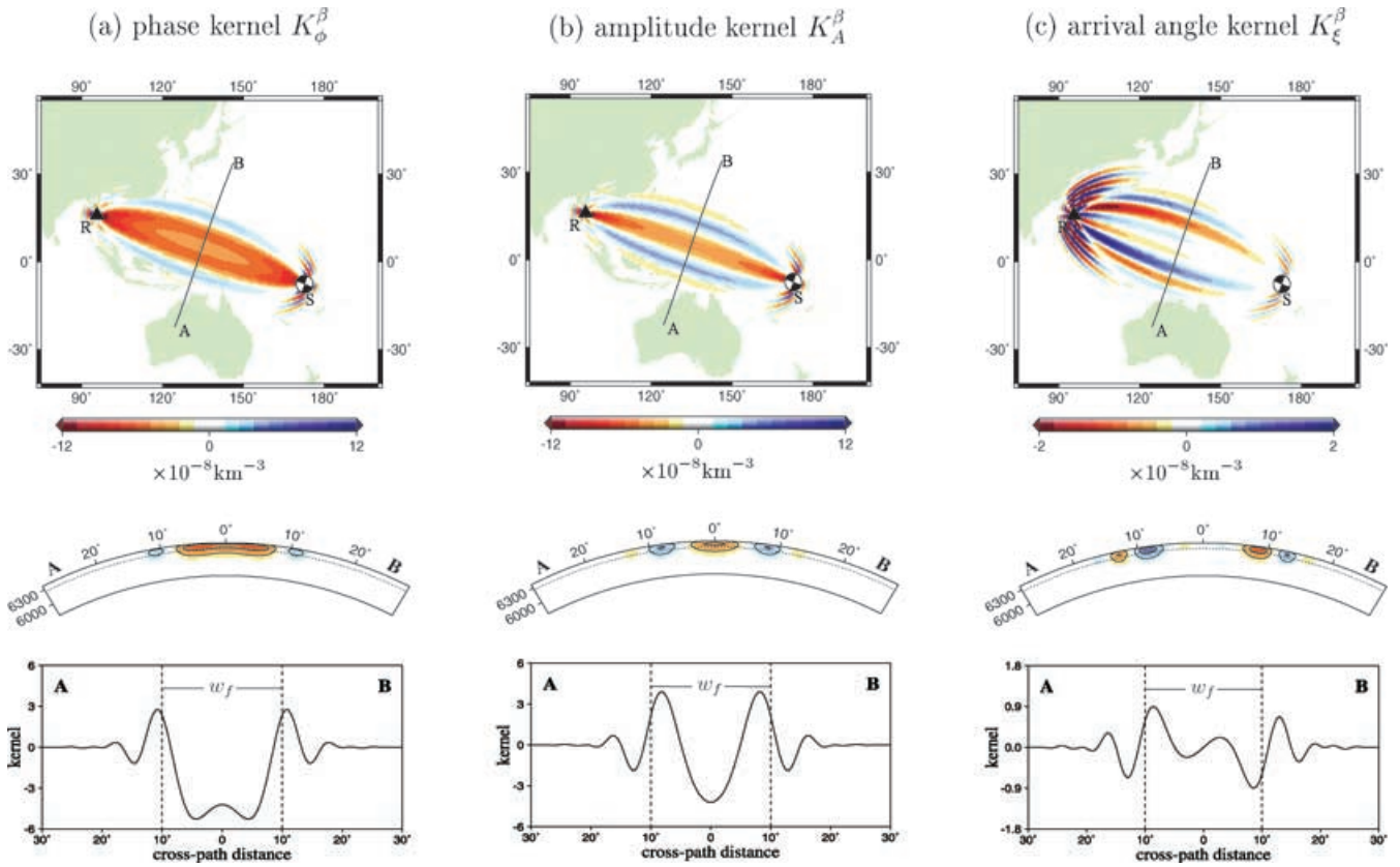
Figure 4. 3-D sensitivity kernels K_{\phi}^{\beta} , K_A^{\beta} , K_{\xi}^{\beta} for a 10 mHz Love wave, excited by a 52 km deep strike-slip seismic source (S). Love wave radiation is maximum in the direction of the source–receiver geometrical ray (see beachball symbol). The epicentral distance to the receiver (R) is \Delta = 80^{\circ} . Sensitivity kernels are for 800 s cosine-taper measurements, with the taper centred at the group arrival time predicted by PREM. Top: Map view of kernels at the depth of approximately greatest sensitivity, 108 km. Middle: Slice view of cross-section AB, dotted lines are plotted at 108 km depth. Bottom: AB cross-section at a depth of 108 km; dashed lines indicate the width of the first Fresnel zone, w_f . Mode-coupling effects have been ignored, i.e. \sigma_1 = \sigma_2 = \sigma .
