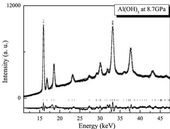
Fig. 4 The LeBail refinement result for XRD pattern of the \text{Al}(\text{OH})_3 high-pressure polymorph at 8.7 GPa, in which R_{wp} = 5.69\% , R_p = 4.10\%
