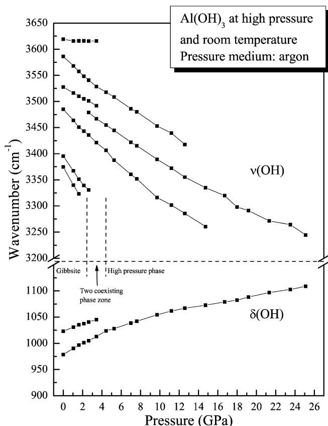
Fig. 6 The pressure dependence of the mode shifts of OH-stretching and deformation modes in Al(OH) 3
