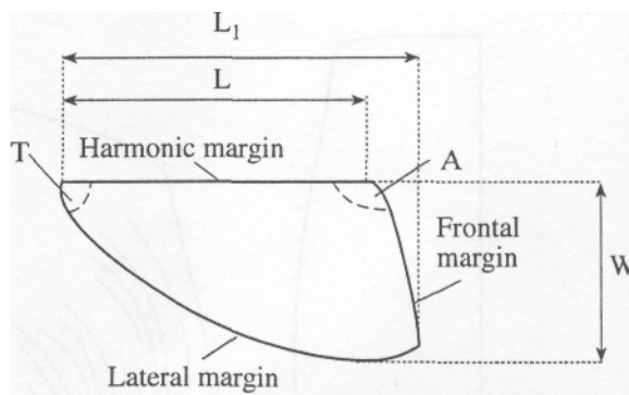
Fig. 2. Measurements of aptychi used in the paper. (A) apical angle, (T) terminal angle, (W) width, (L) length of the harmonic margin, ( L_1 ) length of the aptychus.
