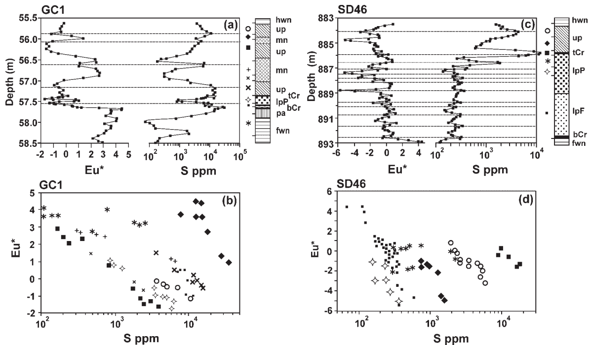
Fig. 14. Variation of Eu^* and S in GC1 and SD46. (a) Variation of Eu^* and S as a function of depth in section GC1. (b) Relative dependence of Eu^* on S over intervals of contiguous samples indicated by the symbols and on the stratigraphic column. (c) As for (a) in section SD46. (d) As for (b) in section SD46. Symbol abbreviations in columns as for Fig. 3. Dashed lines correspond to S peaks.
