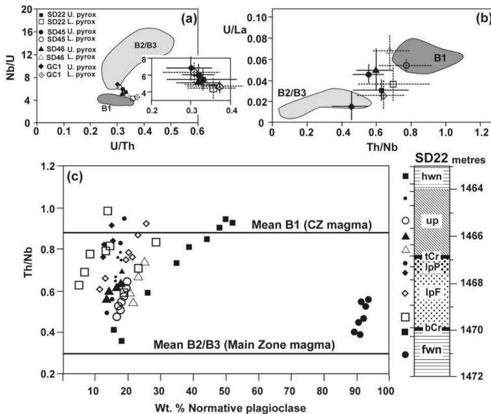
Fig. 5. Incompatible trace element ratios of the four borehole sections compared with the range of inferred Critical Zone (CZ) and Main Zone (MZ) parental magmas of the Bushveld Complex, as represented by B1 and B2/B3 compositions of fine-grained marginal sills (Curl, 2001). (a) Average values and 2\sigma standard deviations for Nb/U and U/Th for the lower pyroxenite (L. pyrox, open symbols and dashed lines) and upper pyroxenite (U. pyrox, closed symbols and continuous lines) in the four sections studied in relation to the fields for parental magma compositions. (b) Average values and 2\sigma standard deviations for U/La and Th/Nb for the lower and upper pyroxenites in the four sections studied in relation to the fields for parental magma compositions. Symbols as for (b). (c) Variation in Th/Nb vs normative plagioclase content for core SD22. Symbol types define a series of arrays for contiguous samples in the vertical profile (same symbols). Compositions for mean CZ and MZ magmas are shown. hwn, hanging-wall norite; up, upper pyroxenite; tCr, top reef chromitite; lpP, lower pegmatoidal feldspathic pyroxenite; lpF, lower feldspathic pyroxenite; bCr, bottom reef chromitite; fwn, foot-wall norite and pyroxene anorthosite.
