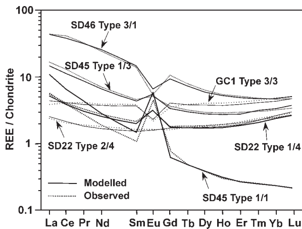
Fig. 11. Observed and modelled REE patterns (Table 4) for a selection of pattern types from each of the sections.
