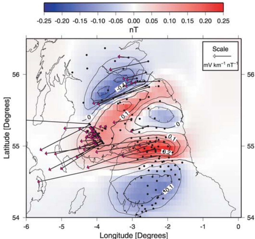
Figure 8. The \mathbf{e}_x telluric vectors recovered via tensor decomposition.
