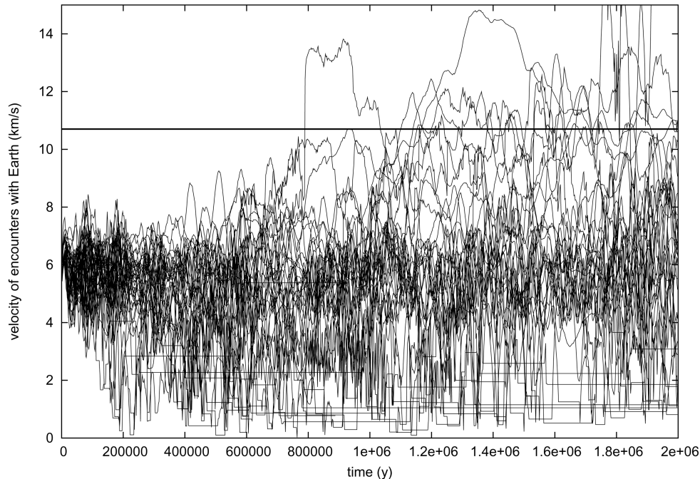
Fig. 2. The time evolution of the relative velocity of encounter with the Earth for 36 objects initially having close encounters at \sim 6 km/s. The horizontal line at 10.7 km/s mark the current value of the encounter velocity for 1996 FG 3 . The horizontal segments at visible in the v_{\text{rel}} < 3 km/s mark the time intervals during which a considered object in not Earth-crossing.
