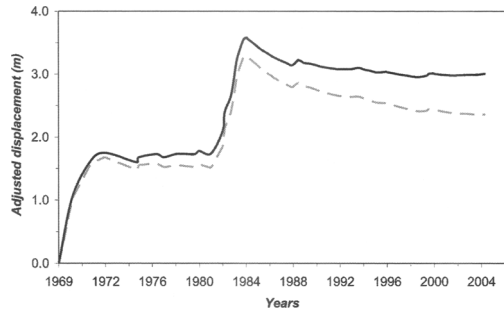
Fig. 8. Adjusted vertical displacement at Serapis between 1969 and 2005 ( solid curve ), after subtracting a background rate of subsidence of 17 mm a -1 (Fig. 7) from the measured deformation ( dashed curve ; Fig. 3). The adjusted curve indicates that no significant movements occurred between 1972 and 1984, and that, by about 2000, the 1982–1984 uplift (of 1.8 m) had decayed by about 0.5 m to a new equilibrium level. The permanent deformation is consistent with magma intrusion from the start of uplift (see also De Natale et al. (2006: this volume pp. 25–45)), whereas the 0.5 m decay may reflect the dissipation of fluids from disturbed aquifers.
