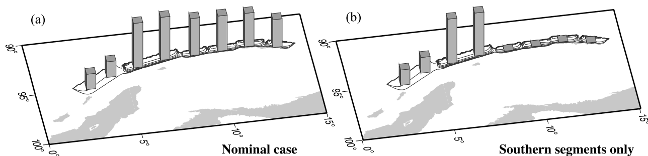
Figure 8. Relative amplitudes of acoustic waves excited at the eight point sources, the centers of uplifted regions by eight fault segments (Figure 1a). (a) Nominal case. They were assumed to be proportional to the average values of uplifts at grid points showing >50 cm uplift. (b) Southern segments only. We also considered an optional model where ruptures in the northern half were too slow to generate acoustic waves.
