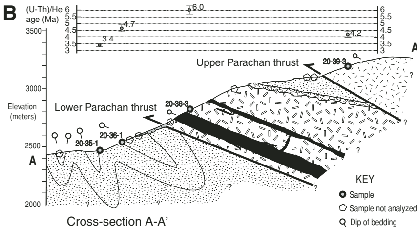
Figure 6. (A) Detailed geologic map of the region around the Dizan (U-Th)-He transect, based on our field mapping. The map shows sample locations relative to surrounding structures and the location of cross-section A-A'. LPT—lower Parachan thrust; UPT—upper Parachan thrust. (B) Cross section A-A', with sample locations and (U-Th)-He cooling ages plotted above the cross section. The lower three samples cross the lower Parachan thrust and indicate slow cooling from 3.4 to 6.1 Ma. This distribution of ages in highly deformed sediments across a thrust suggests that thrusting and synchronous deformation of the footwall rocks were occurring at temperatures above the closure temperature for apatite (~75 °C) and therefore at a depth >~2 km, assuming a 25 °C/km geotherm and a ~25 °C average surface temperature. The hanging wall of the upper Parachan thrust yields a younger 4.2 Ma age, which suggests the possibility that the upper Parachan thrust remained active after activity on the lower Parachan thrust ceased.
