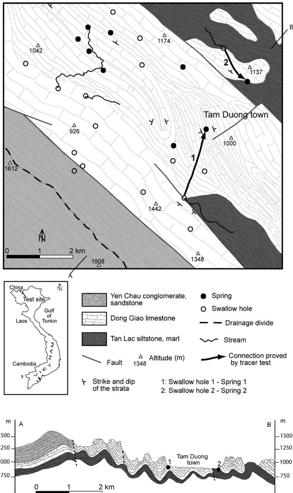
Fig. 3 Location, hydrogeological map and cross-section of the test site
