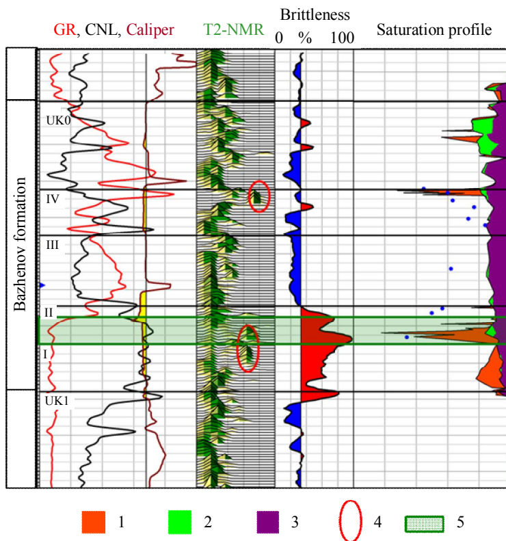
Fig.1. Petrophysical evaluation plot aimed to substantiate perforation intervals hydraulic fracturing initiation points and design of horizontal borehole (1 cell – 1 meter)
