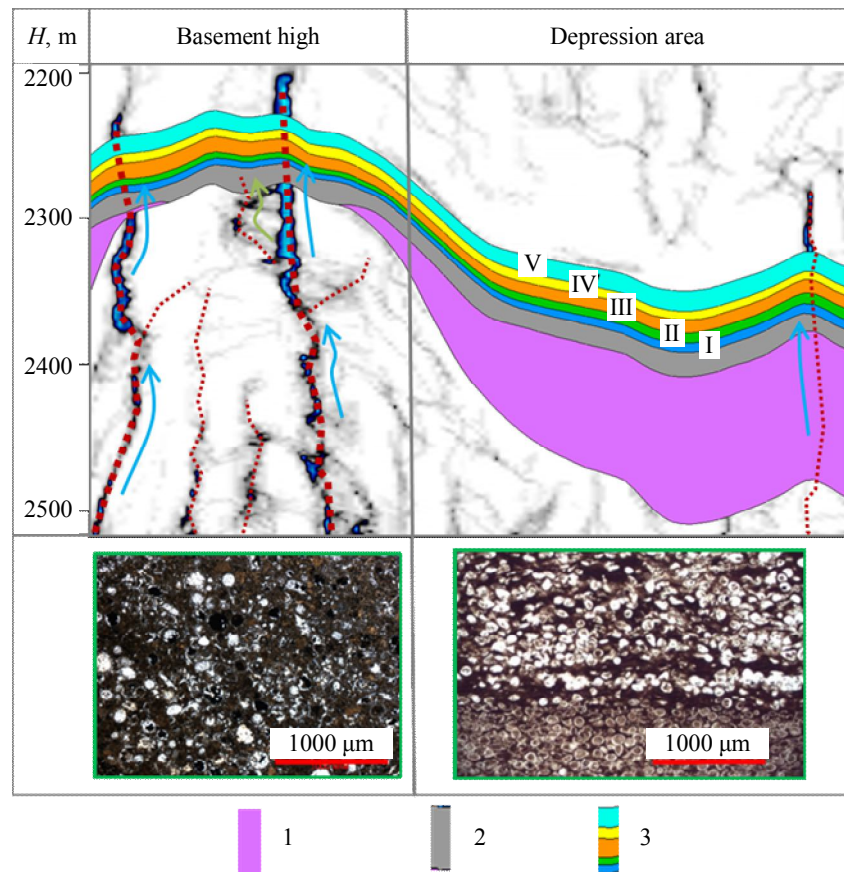
Fig.2. An illustration of a geological concept on a seismic cross-section, built on the technology of ant-tracking [5]
