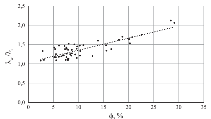
Fig. 3. Collection 1. Linear correlation between the values of the ratio of thermal conductivity of water-saturated and dry samples ( \lambda_w/\lambda_s ) and their porosity. The linear regression equation: \lambda_w/\lambda_s = 1.04 + 0.03 \phi ( R^2 = 0.69 ; N = 54 )
