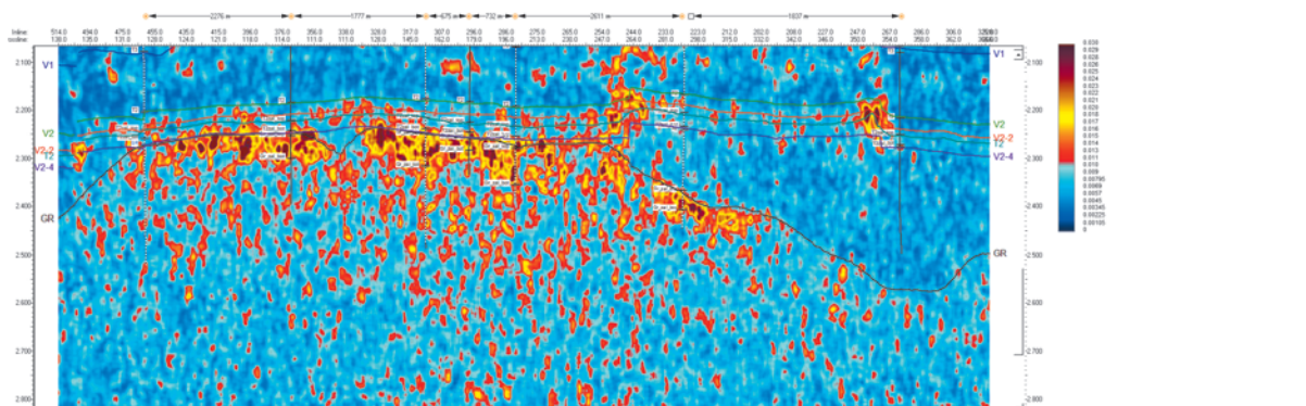
Fig. 7. Time section of scattered waves through wells. Identification of healed faults and faults with open fracturing
