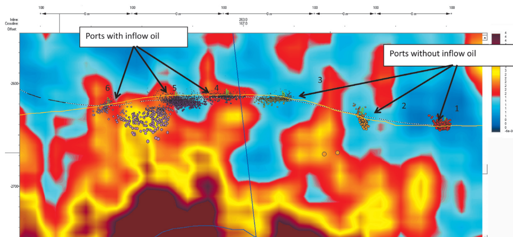
Fig. 13. Fragment of a time section for scattered waves cube projecting the micro-seismic events cloud
