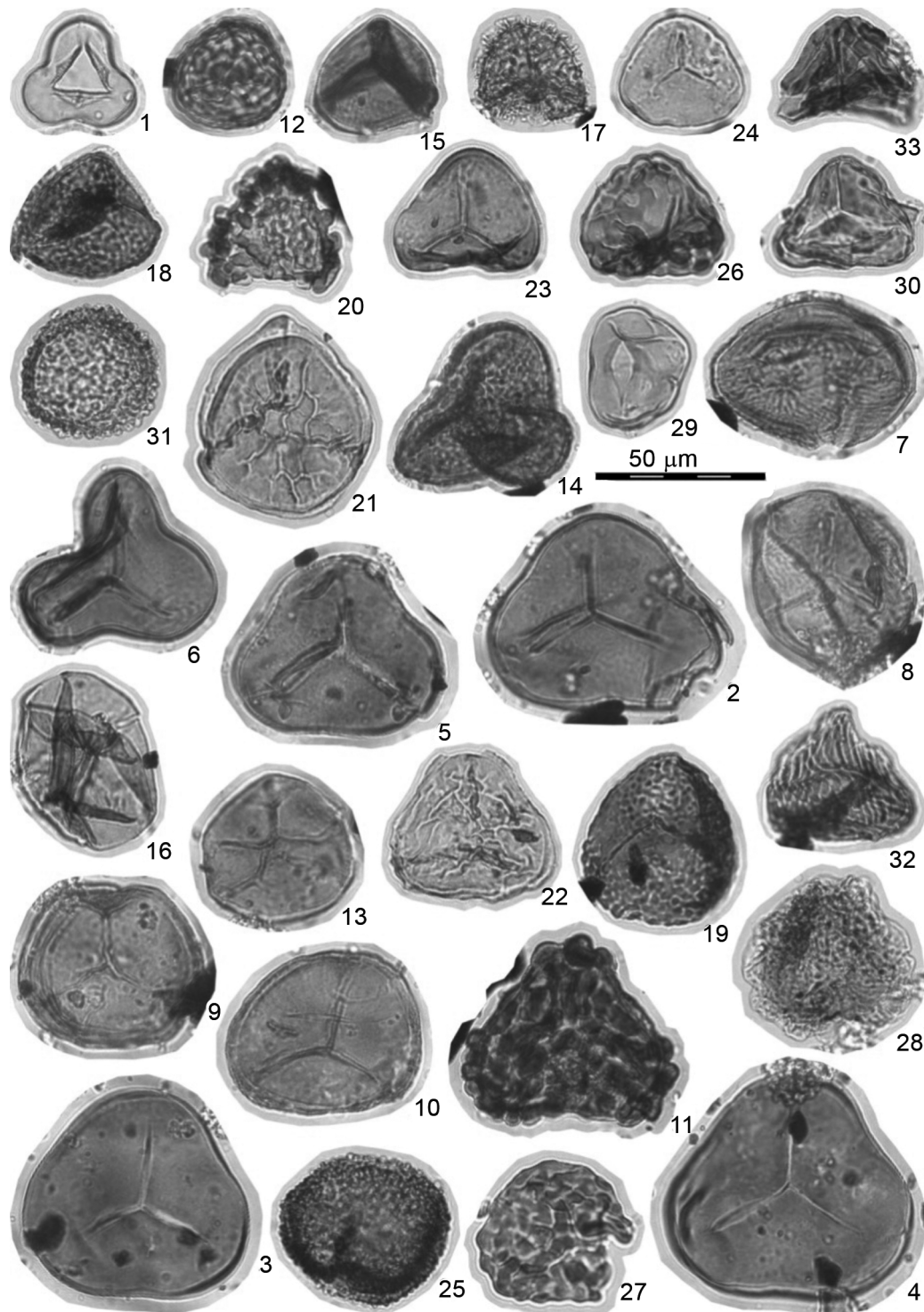
Plate I. 1 – Cyathidites minor Coup., 1953, Sample: yn-001; 2–5 – Concavissimisporites asper Pocock, 1962, Sample: yn-001; 6 – Concavissimisporites sp., Sample: yn-001; 7–8 – Nevesisporites radius (Chlon.) Sriv., 1972, Sample: yn-001; 9–10 – Densoisporites microrugulatus Brenner, 1963, Sample: yn-001; 11 – Cibotioidites arlii Sriv., 1975, Sample: yn-001; 12, 14 – Leptolepidites tenuis Stanl., Sample: yn-001; 13 – Triporoletes reticulatus (Pocock) Ployford, 1971, Sample: yn-001; 15 – Toroisporis sp., Sample: yn-001; 16 – Punctatisporites sp., Sample: yn-003; 17 – Retitriletes reticulispores (Rouse) Krutzsch, 1963, Sample: yn-004; 18–19 – Dictyotriletes samoilovitchae Griazeva, 1965, Sample: yn-004; 20 – Multinodisporites sp., Sample: yn-004; 21–22 – Trochicola sp., Sample: yn-004; 23 – Biretisporites sp., Sample: yn-004; 24 – Cyathidites minor Coup., 1953, Sample: yn-004; 25 – Osmundacidites sp., Sample: yn-004; 26–27 – Klukisporites sp., Sample: yn-006; 28 – Gabonispors labyrinthus Sriv., 1972, Sample: yn-006; 29 – Laevigatosporites ovatus Wils. et Webst., Sample: yn-006; 30 – Gleicheniidites sp., Sample: yn-006; 31 – Gabonispors bacaricumulus Sriv., 1972, Sample: yn-007; 32 – Cicatricosisporites dorogensis Pot. et Gell., 1965, Sample: yn-011; 33 – Cicatricosisporites pseudoaurifer (Bolch.) Li, 1979, Sample: yn-003.
