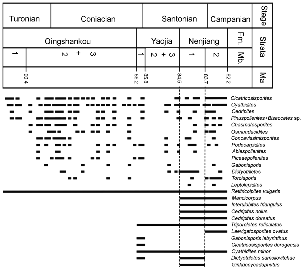
Fig. 4. The geological ranges of the palynological taxa from the lower Yong'ancun Formation and Songliao Basin (Sk1).
