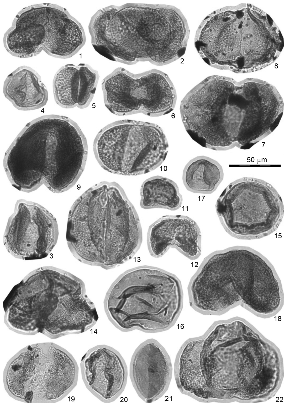
Plate III. 1–2 – Pinuspollenites sp., Sample: yn-001; 3 – Abietinaepollenites pactovae (Krutzsch) Zhang comb.nov., Sample: yn-001; 4, 17, 20 – Phyllocladites inchoatus (Pierce) Norris, 1967, Sample: yn-001; 5 – Podocarpidites minisculus Singh, 1964, Sample: yn-001; 6 – Podocarpidites sp., Sample: yn-001; 7 – Podocarpidites nageiaformis (Zakl.) Krutzsch, 1971, Sample: yn-001; 8 – Piceapollenites sp., Sample: yn-001; 9 – Cedripites dorsatus Gao et Zhao, 1976, Sample: yn-001; 10 – Alisporites bilateralis Rouse, 1959, Sample: yn-001; 11–12 – Cedripites nolus (Gao et Zhao) Sun et He, 1980, Sample: yn-001; 13 – Pseudopicea magnifica Bolch., 1956, Sample: yn-001; 14 – Abiespollenites sp., Sample: yn-001; 22 – Abiespollenites sp., Sample: yn-011; 15 – Araucariacites australis Balme, 1957, Sample: yn-001; 16 – Psophosphaera sp., Sample: yn-004; 18 – Cedripites densireticulatus (Zauer) Krutz., 1971, Sample: yn-004; 19 – Alisporites bilateralis Rouse, 1959., Sample: yn-004; 21 – Ginkgocycadophytus sp., Sample: yn-004.
