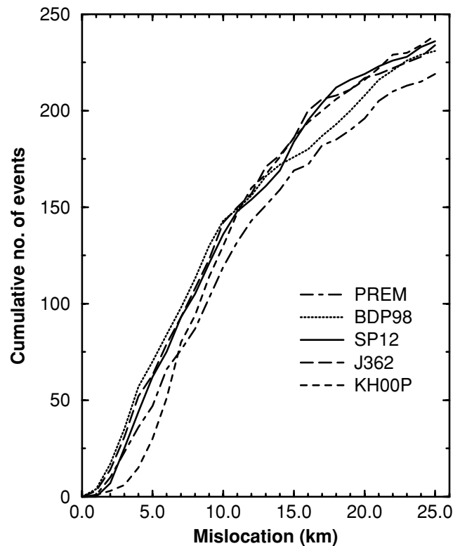
Figure 15. Mislocation statistics for the global reference event database of 246 events. Curves depict the cumulative number of reference events with a mislocation equal to or less than a given value for PREM and four of the models shown in Fig. 15. Models SP12 and J362 give a similar mislocation distribution, but the higher-resolution models show fewer events located with high precision (KH00P) or more events located with lower precision (BDP98).
