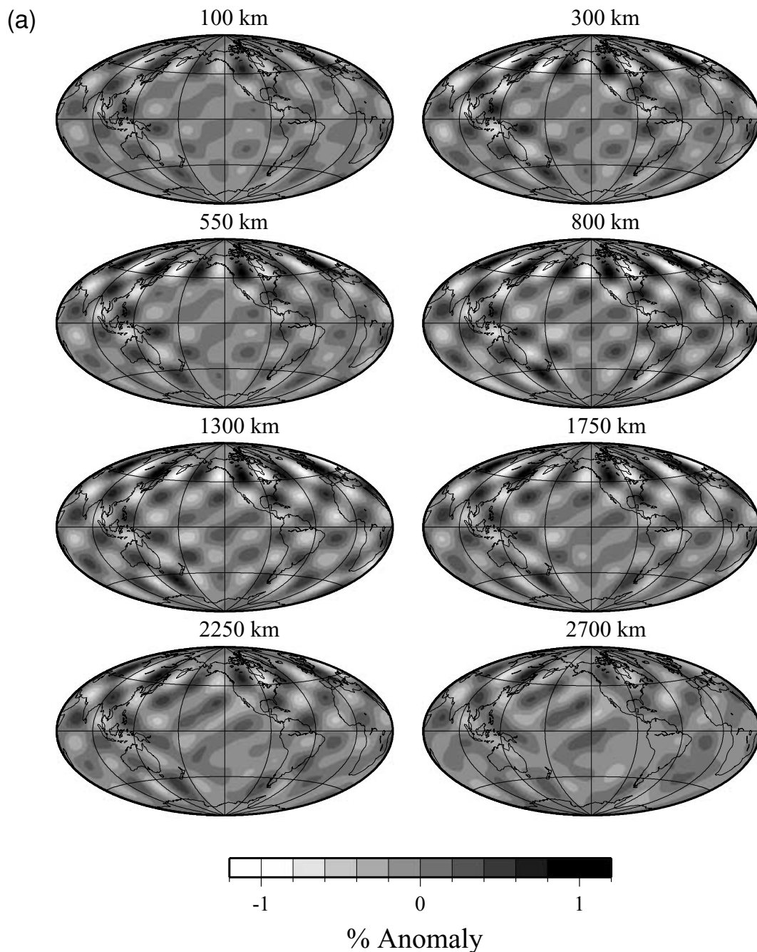
Figure 11. Recovered (a) P and (b) S velocity models at eight depths for resolution test 2. Input model for this test was null for S velocity. Note the much smaller-amplitude scale for (b).
