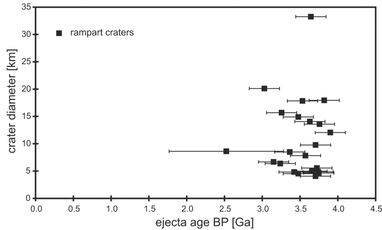
Fig. 6. Absolute model ages of rampart craters versus crater diameter of the Vallis Marineris region. Error bars are 30% for absolute model ages younger than 3 Gyr and \pm 200 Myr for absolute model ages \geq 3 Gyr (Neukum et al. 2004a).
