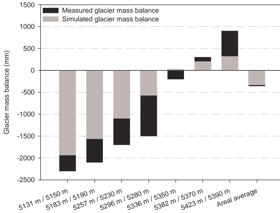
Fig. 3. Comparison of simulated glacier mass balances with the TAC D model and measured glacier mass balances at different altitudes on Yala glacier from 19 May 1996 to 6 October 1996 (Fig. 1). The black bars are behind the gray bars and both start at 0.00 mm. First numbers of x-axis are the altitudes of the 200×200 m 2 cells in which the balance was measured. Second numbers show the altitudes of the observation points.
