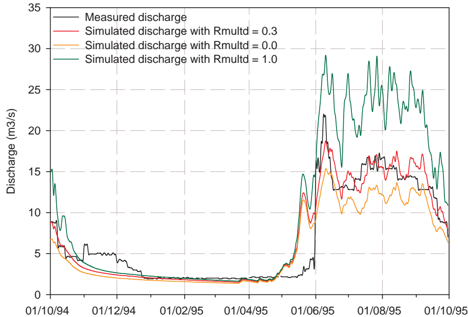
Fig. 7. Sensitivity of the parameter R_{multd} , Langtang Khola catchment.
