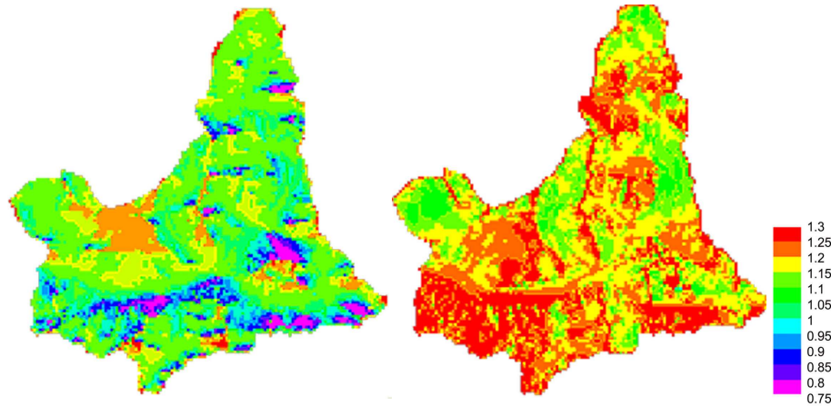
Fig. 6. Spatial distribution of the correction factor for the degree-day method R_{\text{expMap}} (–) at the winter solstice (21 December, left) and the summer solstice (21 June, right).
