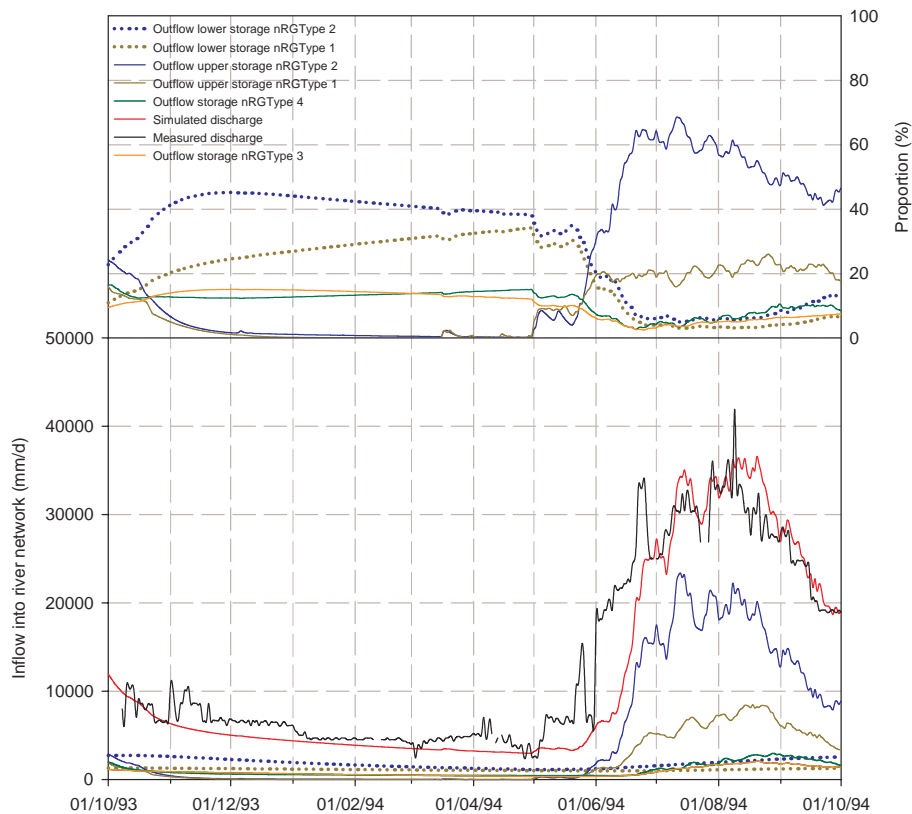
Fig. 8. Contribution of each runoff component to the entire runoff in percent of the entire runoff (upper graphic) and as absolute values (lower graphic) for the hydrological year 1993/94, Langtang Khola catchment.
