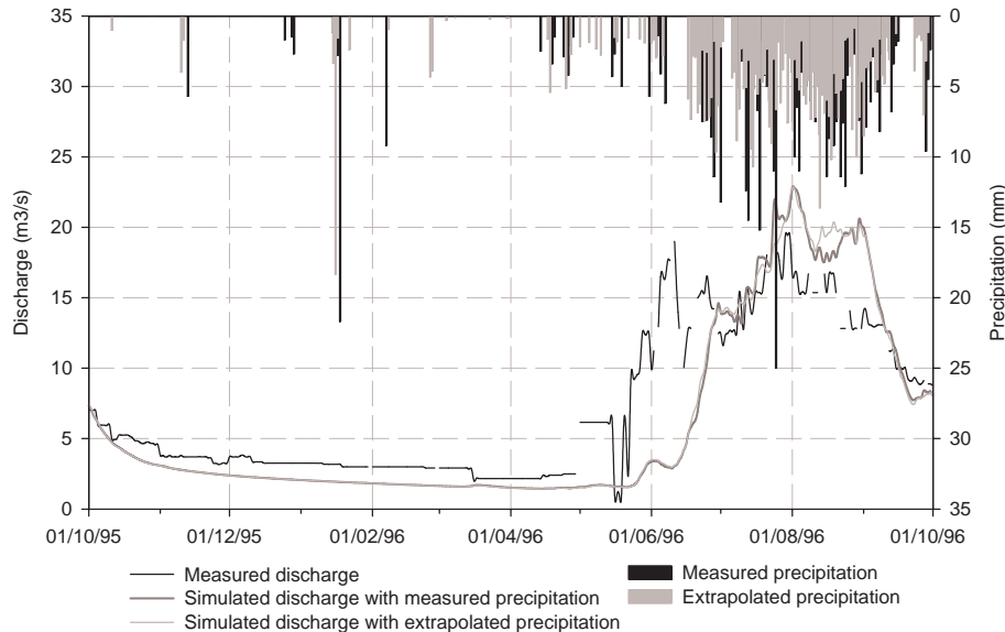
Fig. 5. Comparison of the influences of different precipitation inputs on the discharge simulation. The hydrological year 1995/96 was chosen because of the data availability.
