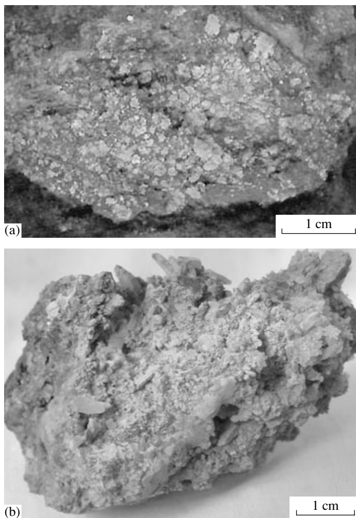
Fig. 7. (a) Pyrite–marcasite mineralization in black silicified dolomite; (b) druse of fine crystalline quartz in cavernous jasperoid at the Alshar deposit.
