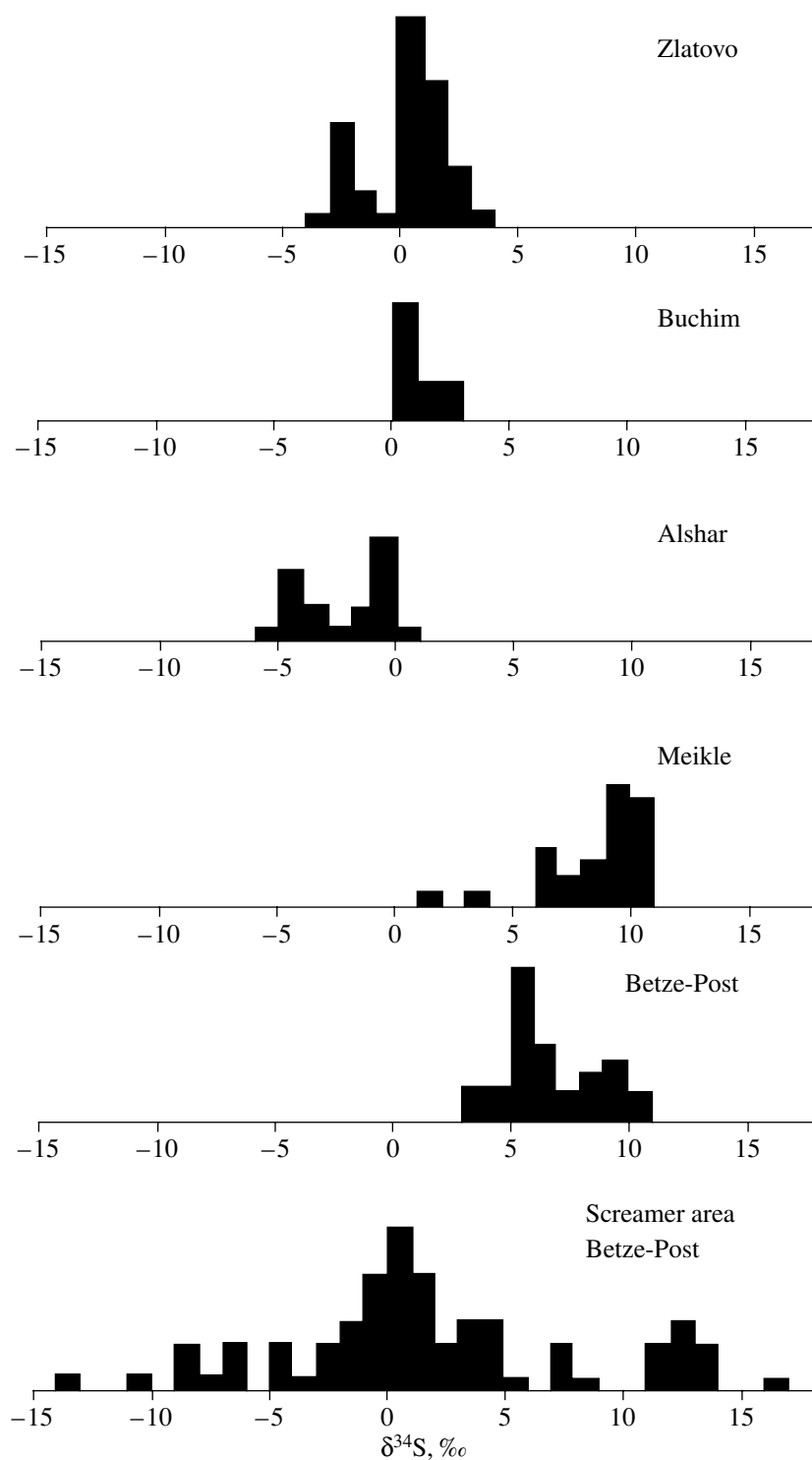
Fig. 11. Sulfur isotopic composition of sulfides from Au-bearing porphyry copper and Carlin-type deposits after Radtke et al. (1980), Serafimovski et al. (1996), Emsbo et al. (2003), and Kesler et al. (2003).
