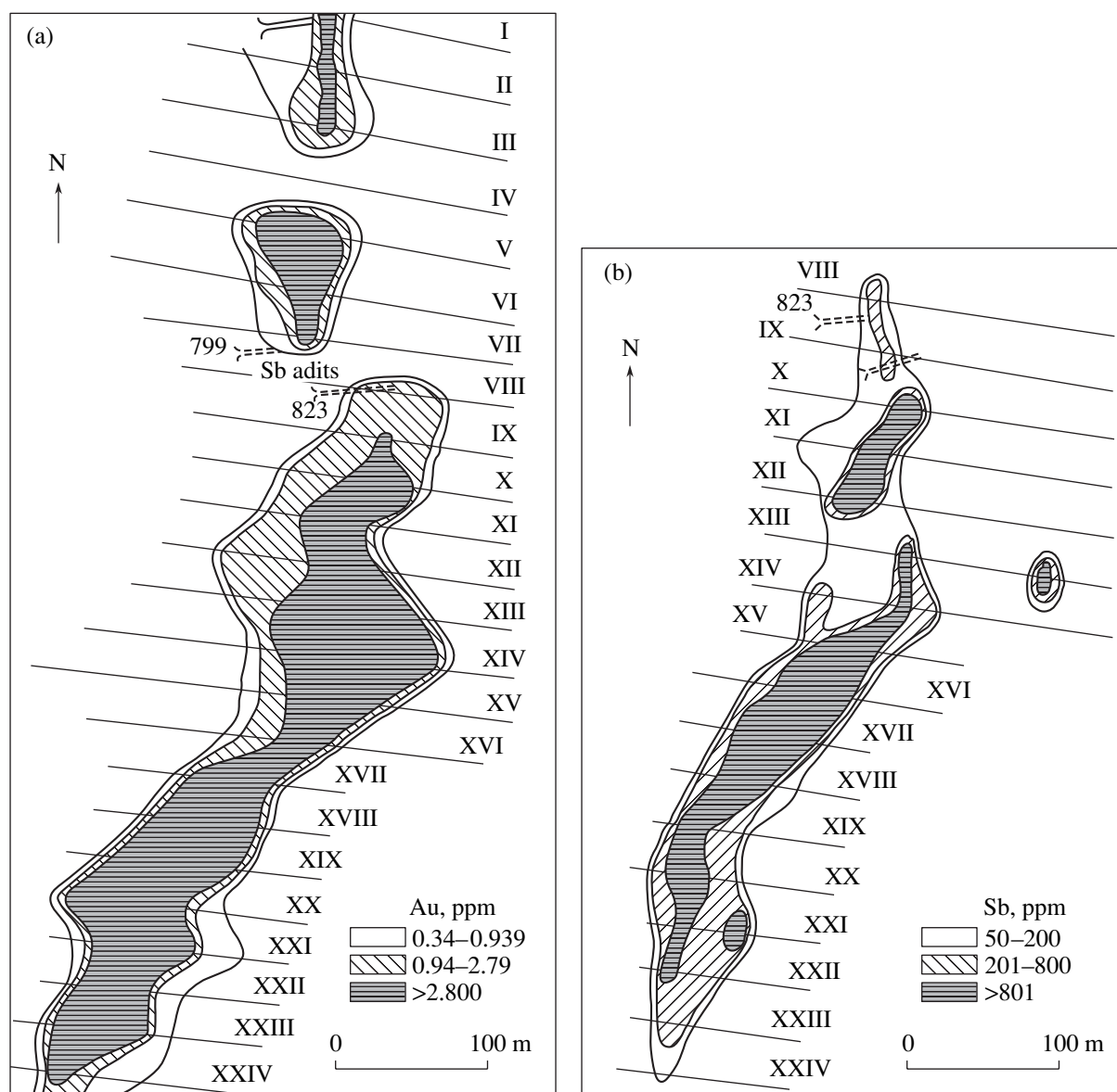
Fig. 6. Geochemical anomalies of (a) Au and (b) Sb in the central area of the Alshar deposit (Hadzi-Petrusev, 1987). The contour of the area is shown in Fig. 3.
