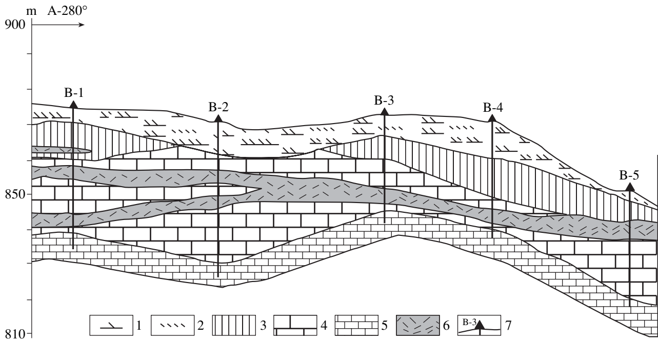
Fig. 5. Geological section across the Alshar deposit along drilling profile 1. (1, 2) Humus; (3) argillization (kaolinization and sericitization); (4) siliceous dolomite; (5) unaltered dolomite; (6) ore zone; (7) borehole and its number.
