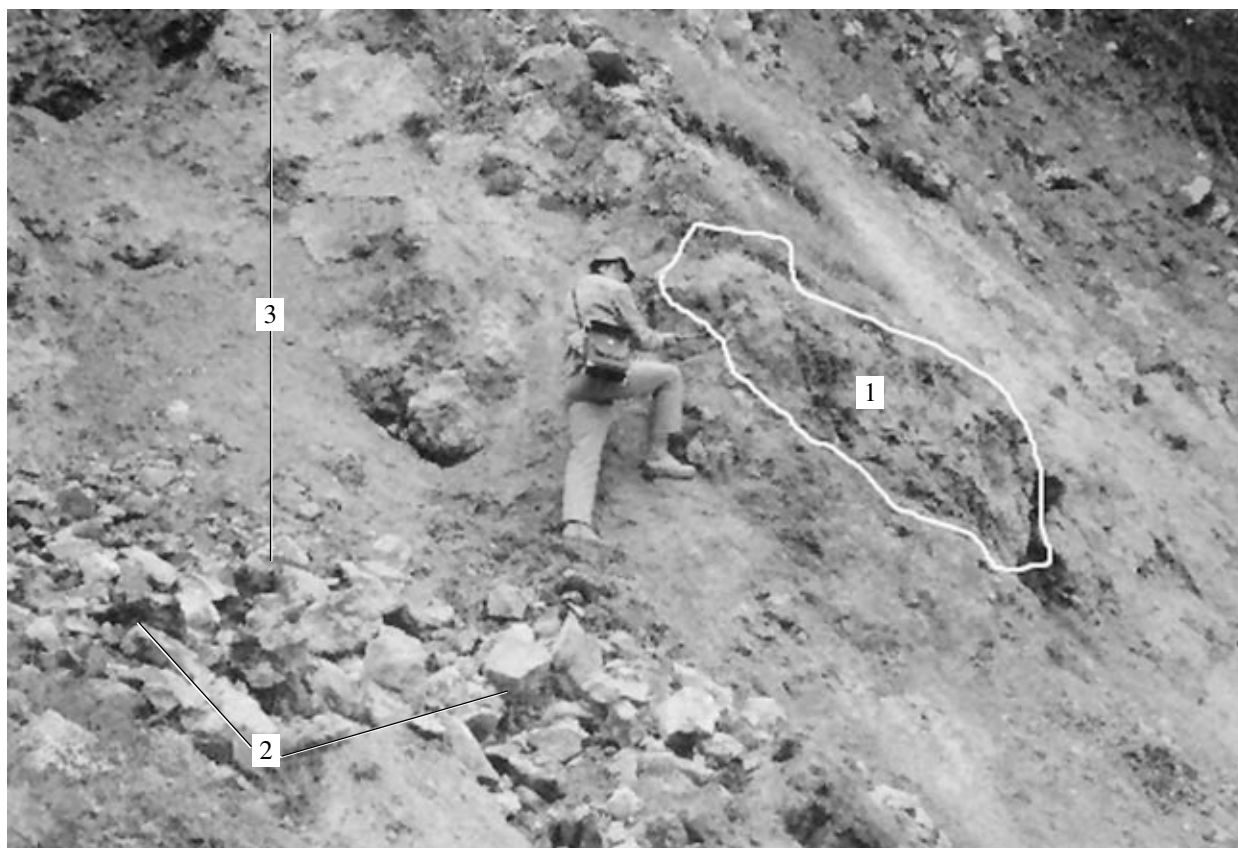
Fig. 8. Zone of argillic alteration with realgar-orpiment mineralization, an outcrop in the southern part of the Alshar deposit. (1) Realgar; (2) jasperoid; (3) zone of argillic alteration.
