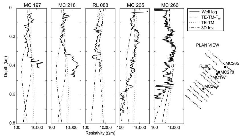
Figure 12. Comparison of borehole-log resistivity data (from Mwenifumbo et al., 2004) and inversion of 2D and 3D models.
