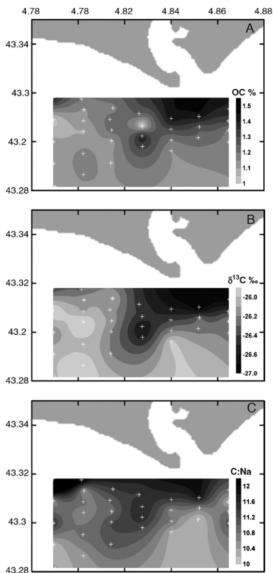
Fig. 6. Contour maps of organic carbon (A), \delta^{13}\text{C} (B) and C:N atomic (C) of surficial sediment in the Rhône prodelta area. Station locations are indicated by crosses.
