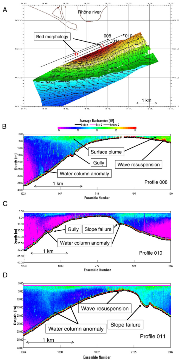
Fig. 1. (A) Tracks and track directions of backscatter ADCP profiles off the Grand Rhône mouth, November 2003. The general morphology of the slump features is outlined; (B) profile 8; (C) profile 10; and (D) profile 11. The positions of anomalies in the water column close to the sea bed are indicated, together with the position of the surface hyperpycnal plume. Areas of high backscatter on the delta top are probably caused by wave resuspension. Bed features were interpreted during a geomorphologic study of the delta front (for further details, see Maillet et al., 2006-this volume).
