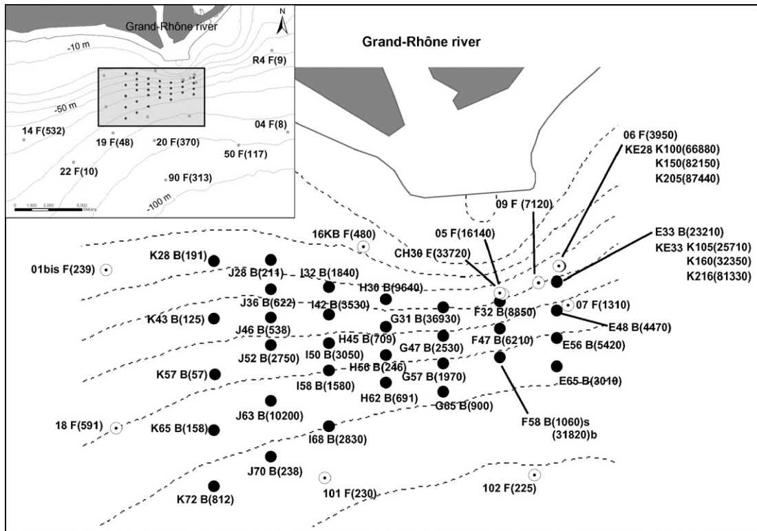
Fig. 2. Location of coring sites off the Grand Rhône River. White dots indicate sites sampled in February–March 2004 and black dots correspond to sites sampled in October 2004. Values in parenthesis are ppm of methane. ‘F’ indicates samples taken with a Fluchat core and ‘B’ indicates Box core samples. Bathymetric lines contour every 10 m. The rest of surveyed sites is shown in inset.
