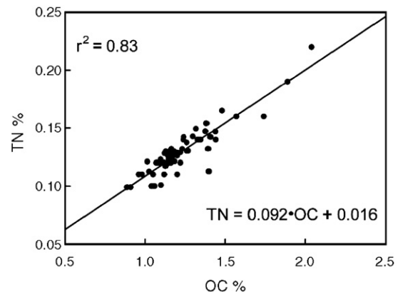
Fig. 5. Relationship between OC% (organic carbon) and TN% (total nitrogen) for surficial and bottom sediments from box-corer.
