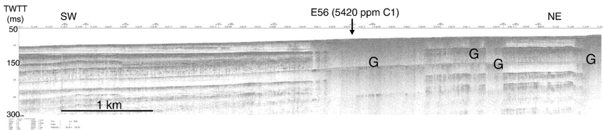
Fig. 4. Seismic line STR-100 off the Rhône outlet. Acoustic anomalies, potential indicators of shallow gas, are indicated with a 'G'. Site E56 was box cored yielding 5420 ppm of methane (see profile location in Fig. 3).
