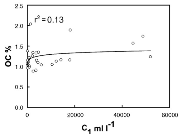
Fig. 8. Relationship between OC% and \text{C}_1 \text{ ml l}^{-1} for bottom samples from box-corer.
