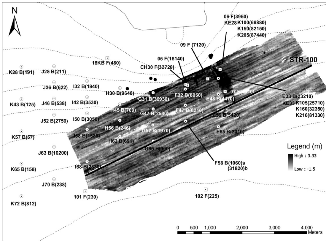
Fig. 3. Coring sites and IFREMER swath model indicating the extension of the sedimentary '03 flood-related deposits (see Maillet et al., 2006-this volume); maximum sedimentary deposition up to 3 m. 'F' indicates samples taken with a Fluchat core and 'B' indicates Box core samples. Values in parenthesis are ppm of methane. Location of seismic line STR-100 is also shown.
