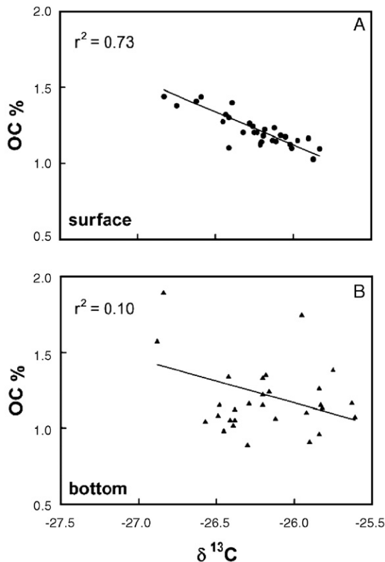
Fig. 7. Relationship between OC% and \delta^{13}\text{C} for (A) surficial and bottom sediments from box-corer (B) collected in the prodelta Rhône area. The OC content in the uppermost and the lowermost layers are differently correlated with the \delta^{13}\text{C} due to the dissimilar degradation rates or the selective remineralization among the isotopes ^{13}\text{C} and ^{12}\text{C} .
