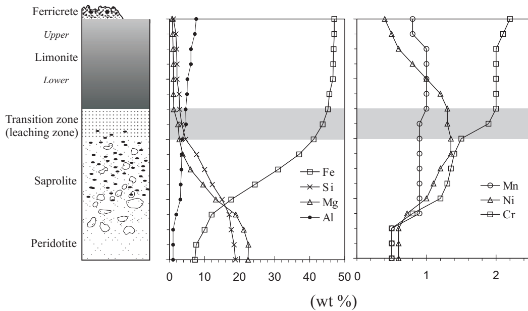
FIGURE 8 | Schematic laterite profile developed on eastern Cuba ultramafic rocks, showing the variation in chemical composition through each zone (from Rodríguez-Pacheco et al., 2003).
