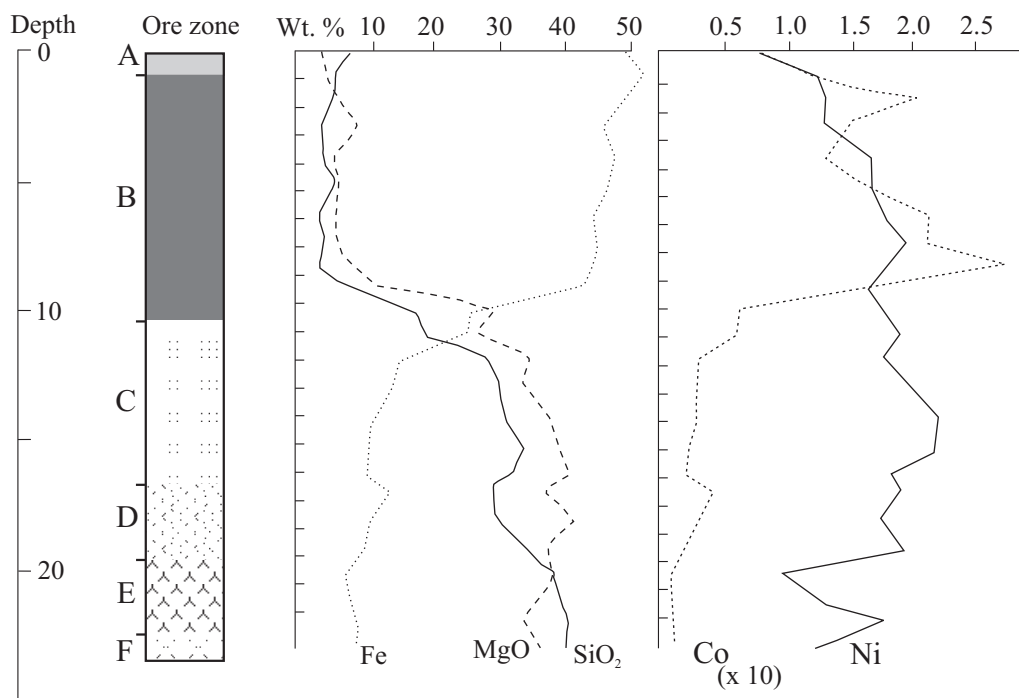
FIGURE 7 | Variation in chemical composition through a nickel laterite from Loma Caribe, Dominican Republic. Courtesy of Falconbridge Dominicana.
