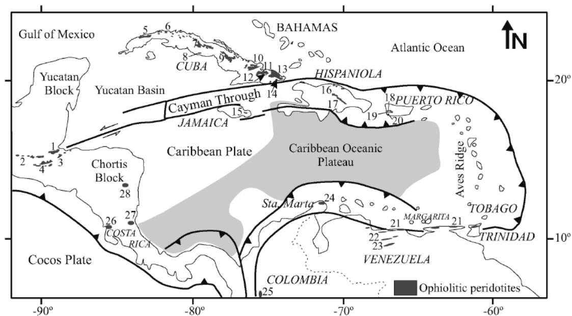
FIGURE 1 | Distribution of ophiolite-related ultramafic rocks around the margins of the Caribbean Plate: 1: Sierra de Santa Cruz; 2: Baja Verapaz Unit; 3: Juan de Paz; 4: El Tambor Group (South Motagua and North Motagua); 5: Cajalbana; 6: Habana-Matanza; 7: Villa Clara; 8: Escambray; 9: Camagüey; 10: Holguín; 11: Mayarí-Cristal; 12: Alto de La Coreia; 13: Moa-Baracoa; 14: Sierra del Convento; 15: Arntully; 16: North Coast Belt; 17: Loma Caribe; 18: Monte del Estado; 19: Río Guanajibo; 20: Bermeja; 21: La Franja Costera; 22: Loma de Hierro; 23: Villa de Cura; 24: Guajira Peninsula (serpentinites of Cabo de la Vela); 25: "Dunita de Medellín" (Aburrá ophiolite); 26: Santa Elena; 27: Río San Juan; 28: Siuna. Main localities are numbered in italics.
