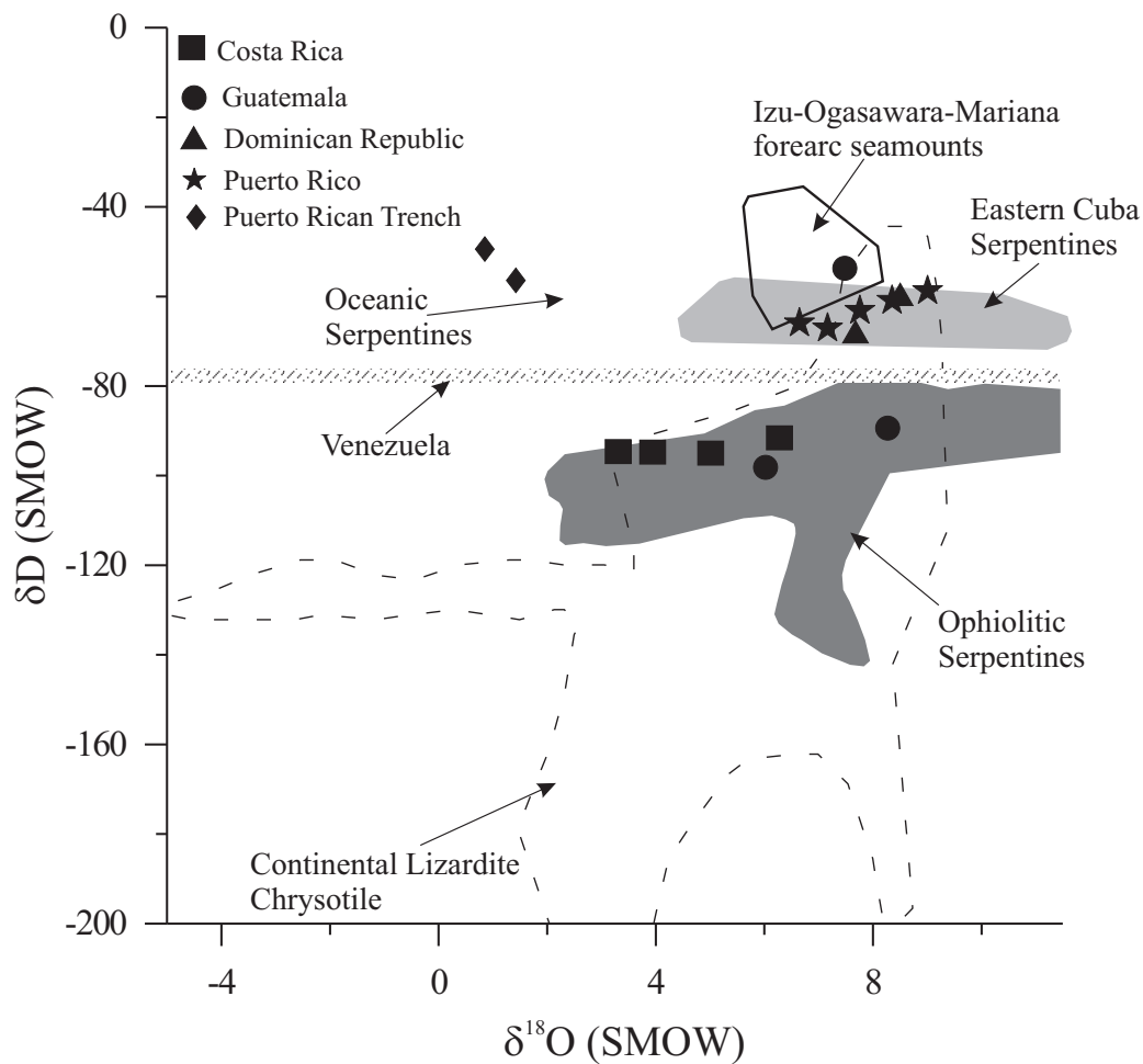
FIGURE 4 | a, \delta D versus \delta^{18}O plot of Caribbean serpentine. The isotopic values of serpentine from Venezuela, Costa Rica, Guatemala, Dominican Republic, Puerto Rico and Puerto Rican Trench are taken from Wenner and Taylor (1973, 1974). The isotopic domains are from: "oceanic serpentine" and "ophiolite serpentine" (Wenner and Taylor, 1973), "continental serpentine" (Wenner and Taylor, 1974), Izu-Ogasawara-Mariana forearc serpentines (Sakai et al., 1990), eastern Cuba serpentine (Proenza et al., 2003a).
