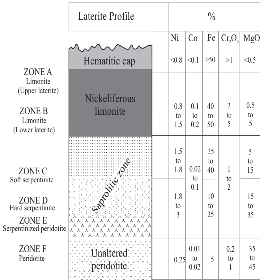
FIGURE 5 | Nickel laterite soil profile showing the zones and variation in chemical composition in each zone. Loma Caribe, Dominican Republic. Courtesy of Falconbridge Dominicana.
