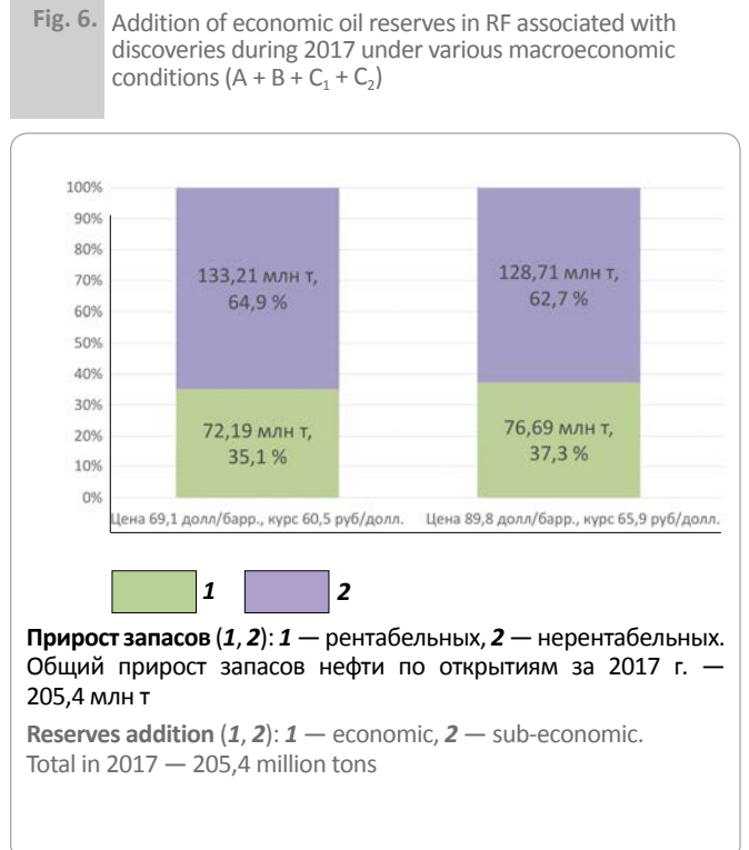
Рис. 6. Прирост рентабельных запасов нефти в РФ по открытиям за 2017 г. при различных макроэкономических условиях (A + B + C 1 + C 2 ) Fig. 6. Addition of economic oil reserves in RF associated with discoveries during 2017 under various macroeconomic conditions (A + B + C 1 + C 2 )
