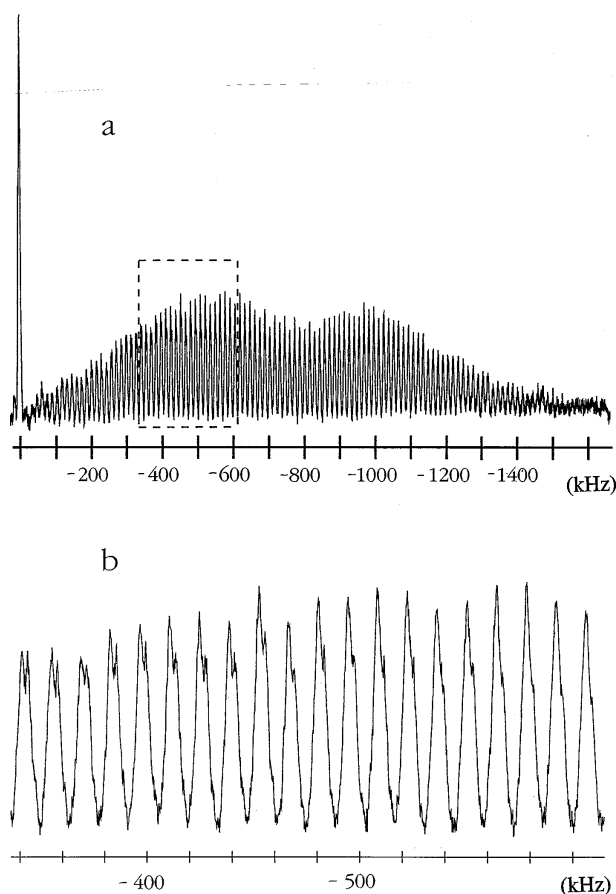
FIGURE 10. (a) The ^{27}\text{Al} NMR experiment of the sample heated at 970\text{ }^{\circ}\text{C} , taken at an offset of -800\text{ kHz} , showing the uncorrected ST envelope. (b) Expansion of the ST spinning sideband region.
