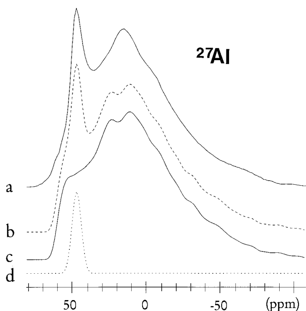
FIGURE 9. The ^{27}\text{Al} CT fit of the spectrum of tsaregorodtsevite heated at 970\text{ }^{\circ}\text{C} . (a) Experimental CT, (b) overall fit, (c) original site, and (d) assumed one site with C_q = 8.5\text{ MHz} and isotropic chemical shift of 62\text{ ppm} .
