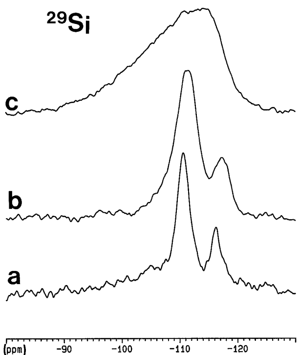
FIGURE 6. The ^{29}\text{Si} MAS NMR spectra of tsaregorodtsevite, (a) unheated (6271 scans), (b) heated at 690^\circ\text{C} (922 scans), and (c) heated at 970^\circ\text{C} (10 177 scans).
