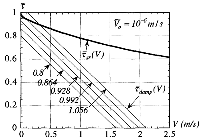
Figure 12. Relative position of the radiation damping line \bar{\tau}_{\text{damp}}(V) to the steady-state strength \bar{\tau}_{\text{ss}}(V) for the enhanced velocity-weakening law, for various \bar{\tau}_0^b , with V_{\text{weak}} = 3.0 m/sec for the enhanced velocity-weakening law. For this case, no intersection can be found if \bar{\tau}_0^b < \bar{\tau}_{\text{pulse}} = 0.974 .
