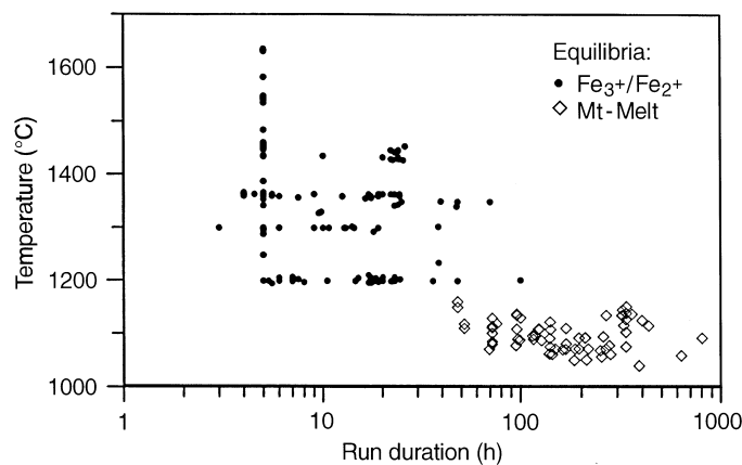
Fig. 3 Temperature – run duration relations for \text{Fe}^{3+}/\text{Fe}^{2+} and magnetite-melt equilibria studies. Two hundred and eighty-nine glasses relevant to \text{Fe}^{3+}/\text{Fe}^{2+} equilibria experiments were used to calibrate empirical equations for the calculations of \text{Fe}^{3+}/\text{Fe}^{2+} ratios in the melt (Sack et al. 1980; Kilinc et al. 1983; Kress and Carmichael 1988, 1991; Borisov and Shapkin 1990; Mysen 1991). The 99 magnetite-melt equilibria points are the same as shown in Figs. 1 and 2
