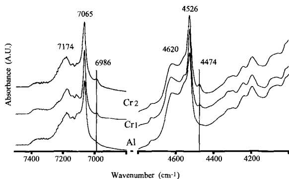
Figure 3. Diffuse reflectance NIR spectra in the 4800–4000- \text{cm}^{-1} and 7500–6800- \text{cm}^{-1} regions of the Cr-bearing kaolinites described in Table 1.
