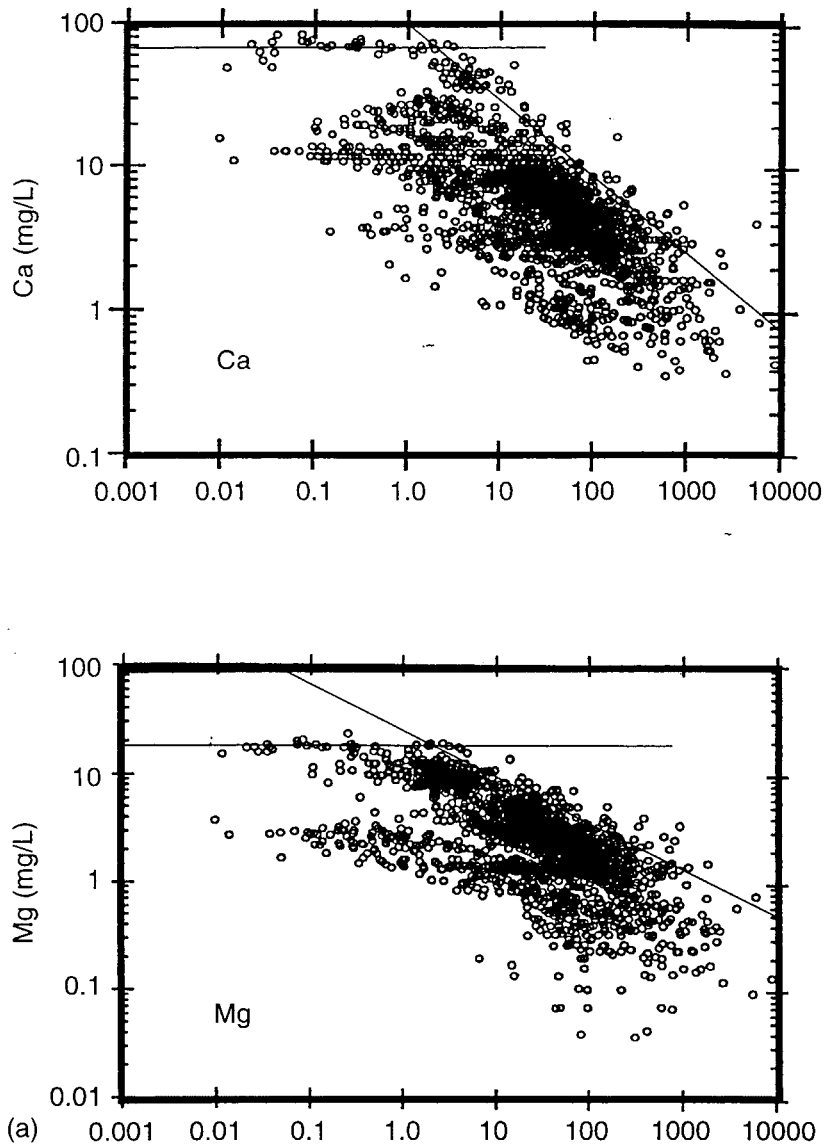
Figure 8 Concentration-discharge relationships for monolithologic basalt catchments of the world. Data are shown for Ca, Mg, K, Na, \text{SO}_4 , and total dissolved solids (TDS). Source of data is Bluth (1990).
