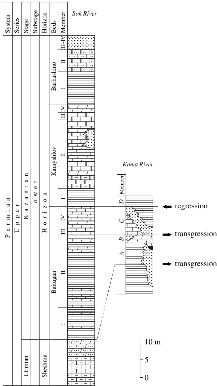
Fig. 7. Correlation scheme for lower Kazanian deposits in the Kama River lower courses and the substage stratotype in the Sok River head, Samarskaya oblast (symbols as in Fig. 2).
