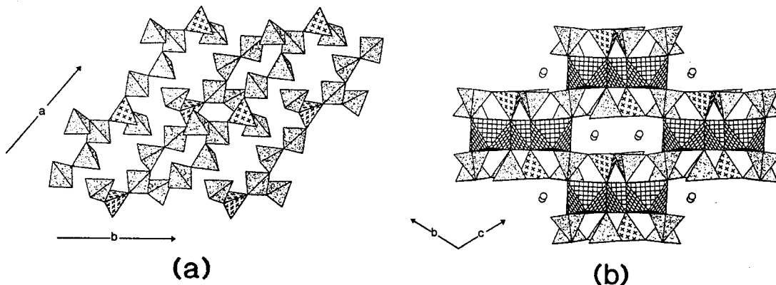
FIG. 4. The crystal structure of "makarochkinite": (a) projected onto (001); note the chains of ( \text{BeO}_4 ) (cross-shaded) and ( \{\text{Si,Al}\}\text{O}_4 ) (random-dot shaded) tetrahedra extending parallel to the a axis; (b) projected onto (100); circles in (b) represent interstitial Ca atoms.
