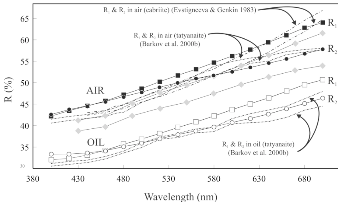
FIG. 5. Reflectance spectra for a taimyrite grain with the composition (\text{Pt}_{1.55}\text{Pd}_{0.60}\text{Cu}_{0.85})_{\Sigma 3}\text{Sn} in air (filled circle and square) and oil (white circle and square). For comparison: published reflectance data for taimyrite (grey diamonds; R_1 and R_2 ; Begizov et al. 1982), tatyanaite (dotted lines; R_1 and R_2 in air and oil; Barkov et al. 2000b) and cabriite \text{Pd}_{2.04}(\text{Sn}_{0.91}\text{Sb}_{0.07})_{\Sigma 0.98}\text{Cu}_{0.98} as broad dashed line (Evstigneeva & Genkin 1983).
