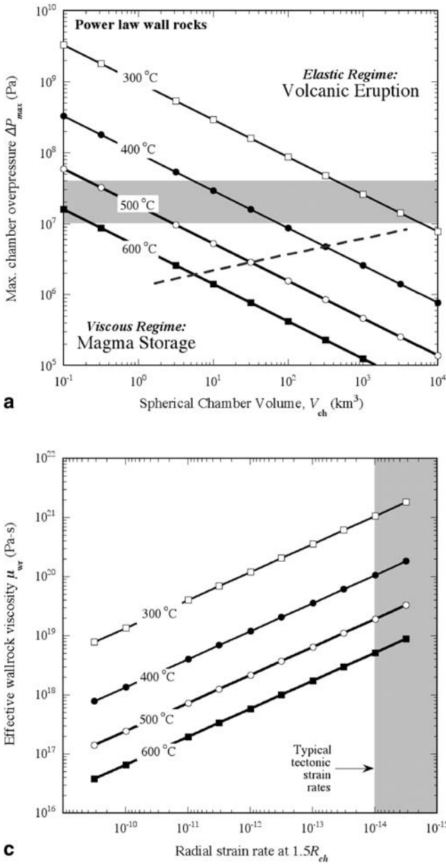
Fig. 5 a The maximum chamber over-pressure, \Delta P_{max} , generated by a constant magma influx, Q=0.005 km 3 year -1 , as a function of chamber volume, V_{ch} , for a spherical chamber contained in wall rocks with a power law rheology. The wall rocks are taken to be Westerly granite with 0.1% water (e.g., Hansen and Carter 1983). In a way similar to Fig. 4, the shaded region shows the probable range of critical dike overpressures, \Delta P_{crit} = 10 - 40 MPa, required to propagate a rhyolite dike to the surface and delineates
