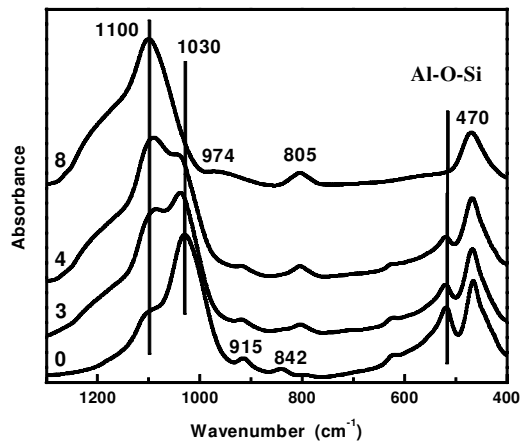
FIG. 2. IR spectra of montmorillonite SAZ-1 treated in 6 M HCl at 80^\circ\text{C} for 0, 3, 4 and 8 h. Data from Madejová et al. (1998).
