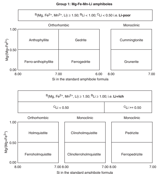
FIGURE 1. Classification of the Group 1 amphiboles; Mg-Fe-Mn-Li amphiboles.
