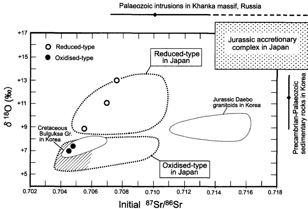
Figure 7 \delta^{18}\text{O} (SMOW) versus initial ^{87}\text{Sr}/^{86}\text{Sr} (at 85 Ma) plot for the representative reduced- and oxidised-type granitoids in southernmost Sikhote–Alin (Fig. 5). Also shown are data areas for granitoids and the Jurassic accretionary complex (metasedimentary rocks from the Ryoke Belt) in Japan (Matsuhisa et al. 1982; Ishihara and Matsuhisa 2002). The oxidised-type granitoids in Japan generally have low initial ^{87}\text{Sr}/^{86}\text{Sr} ratios (hatched), but rarely have high values ( \sim 0.710 ) in the eastern San-in Belt within Southwest Japan (see Fig. 4). Data areas for the Korean granitoids are based on Kim et al. (1992, 1996); Jurassic Daebo (mainly reduced-type) and Cretaceous Bulguksa in the Gyeongsang Basin (oxidised-type), excluding the data for altered rocks. Available data for basement rocks are limited, but their ranges are shown by bars with diamonds of average values: Precambrian to Palaeozoic sedimentary rocks ( \delta^{18}\text{O} = +8.9 to +13.4\text{‰} ( n=3 )) in the southern Korean Peninsula (Kim et al. 1992, 1996) and Palaeozoic gabbro to granitic intrusions (initial ^{87}\text{Sr}/^{86}\text{Sr} = 0.707 to 0.720 ( n=7 )) in the Voznesenka area within the Khanka massif (Ryazantseva et al. 1995).
