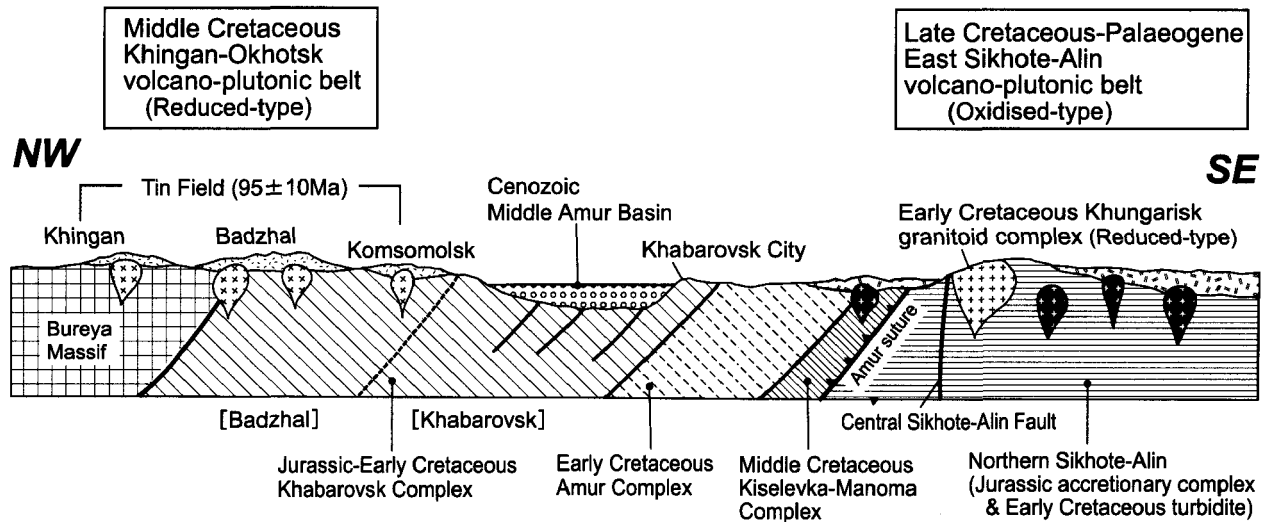
Figure 3 Schematic NW-SE cross section through the Khingan-Okhotsk active margin and northern Sikhote-Alin (Sato et al. 2002); modified from Faure & Natal'in (1992) and Natal'in (1993). Episodic magmatism and mineralisation in the Khingan-Okhotsk Tin Belt ( 95 \pm 10 Ma) is coeval with the middle Cretaceous (Albian-Cenomanian) Kiselevka-Manoma complex (Voinova et al. 1995; Zybrev 1996; Nechaev et al. 1996). The Khungarisk complex a conventional name for a group of Early Cretaceous granitoid plutons in north-central Sikhote-Alin.
