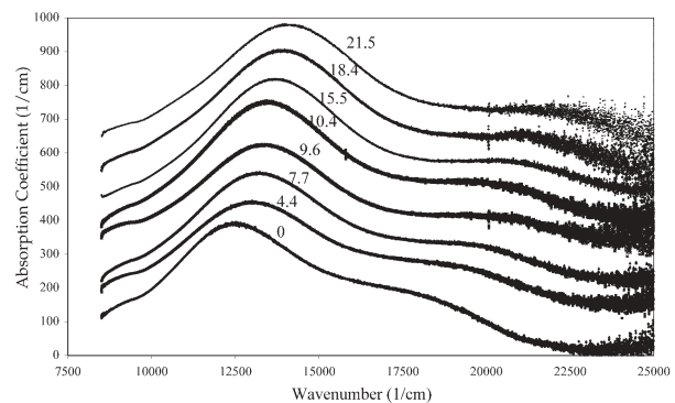
FIGURE 2. High-pressure optical absorption spectra of ringwoodite. Numbers are pressure in GPa.
