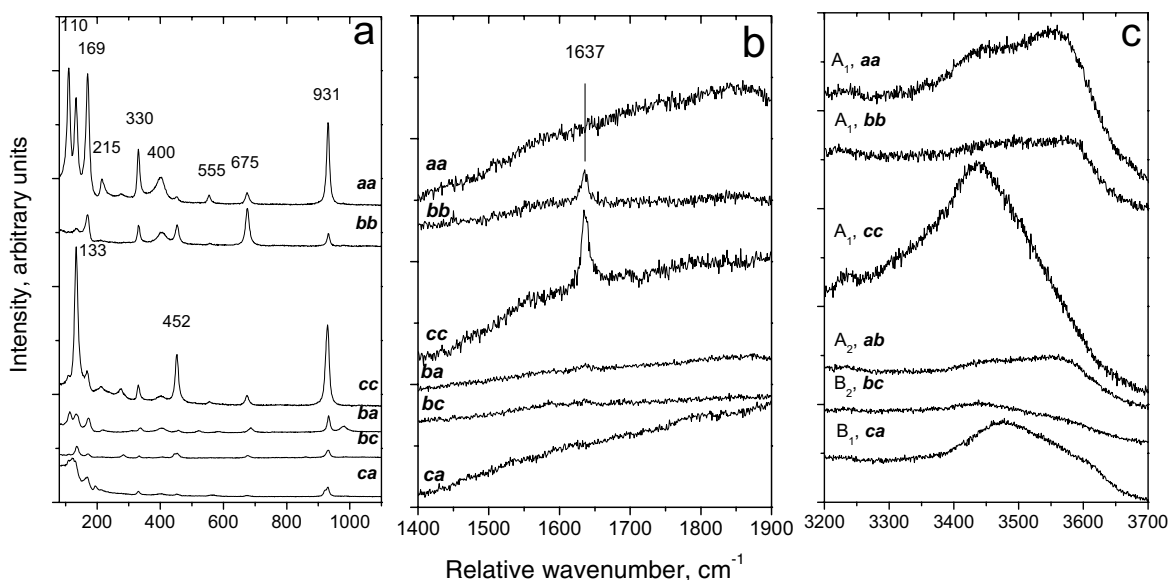
FIGURE 2. Polarized single-crystal Raman spectra of the lattice (a), H 2 O bending (b), and O-H and H 2 O stretching (c) modes in hemimorphite at 295 K.
