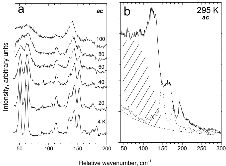
FIGURE 7. (a) A stacked plot of the polarized ac -spectra ( 4 \leq T \leq 100 K) in the low-frequency region of the crystal lattice and H 2 O translational vibrations in hemimorphite. (b) Room-temperature ac -spectra of the natural (top spectrum in solid) and dehydrated (bottom spectrum in dotted) samples. The baseline for both spectra is shown by the dashed curve. The hatched area corresponds to the scattering on external (translational) vibrations of the H 2 O molecule.
