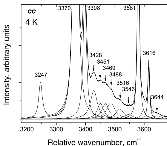
FIGURE 4. Result of curve fitting of the low-temperature cc -spectrum of the H 2 O(I) stretching vibrations in hemimorphite.
