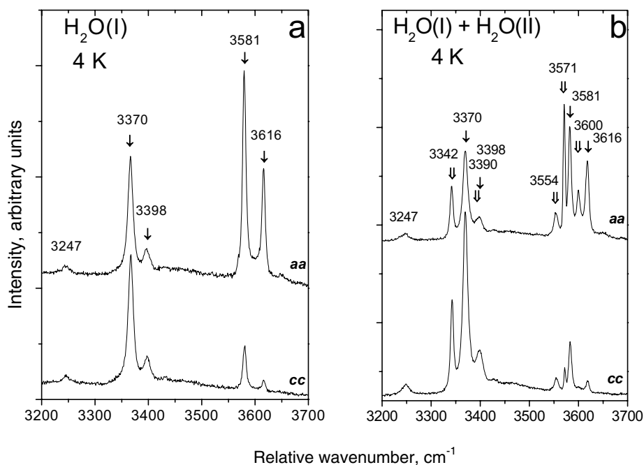
FIGURE 3. Polarized single-crystal Raman spectra of the O-H and H 2 O stretching modes in hemimorphite at 4 K taken in different areas of the crystal surface. The features labeled by single arrows comprise the bands of Set I, which characterize the H 2 O(I) state of the H 2 O molecule and hydroxyl groups in the cavity; double arrows label the bands of Set II, which characterize the H 2 O(II) state. One can see that the spectra represented in a involve only the bands of Set I, whereas the spectra in b involve the bands of both Sets I and II.
