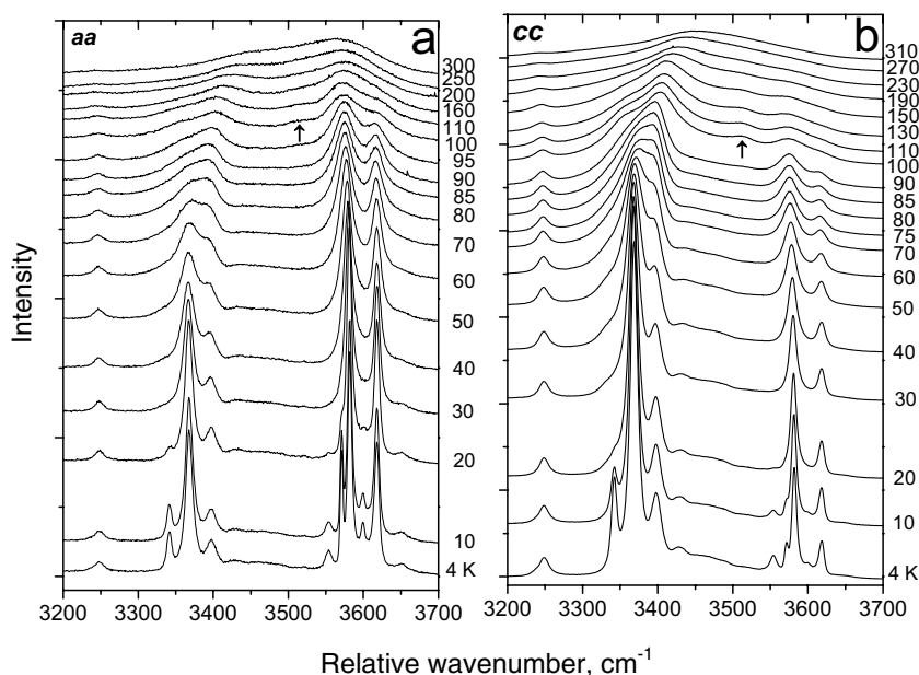
FIGURE 5. Temperature evolution of the polarized spectra showing the O-H and H 2 O stretching modes in hemimorphite; (a) aa -spectra and (b) cc -spectra. The appearance of the new band at around 3500 cm -1 at T \geq 100 K is shown by the arrow.
