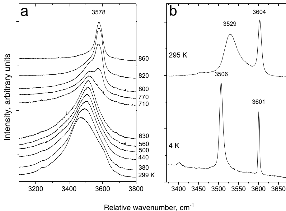
FIGURE 8. The unpolarized spectra of O-H and H 2 O stretching modes in hemimorphite at elevated temperatures (a) and the spectra of O-H stretching vibrations of dehydrated hemimorphite (b).
