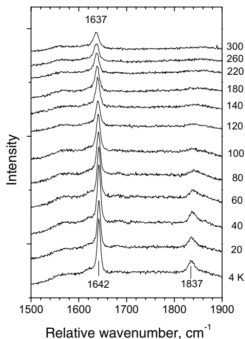
FIGURE 6. The spectra of H 2 O bending vibration vs. temperature.
