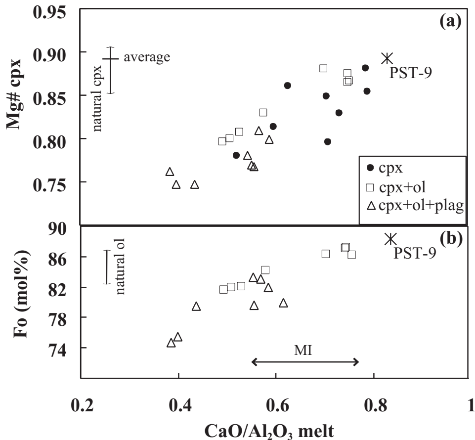
Fig. 6. Mg-number (calculated with \text{FeO}_i ) in experimental clinopyroxenes (a) and Fo in experimental olivines (b) plotted as a function of the degree of differentiation ( \text{CaO}/\text{Al}_2\text{O}_3 ) of coexisting melts. Data for PST-9 are from Table 1. The range of Mg-number in diopsidic clinopyroxene phenocrysts from golden pumice is shown for comparison (source of data as in Fig. 5), together with the average value. Compositions of homogeneous olivines considered to be in equilibrium with the golden pumices ( \text{Fo}_{83-87} , Bertagnini et al. , 2003) and of their melt inclusions (MI) are also indicated.
