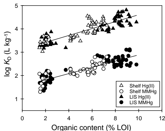
Fig. 5. Variation of the distribution coefficients ( K_D ) of MMHg and Hg(II) with organic content of sediments, measured as percent loss-on-ignition (%LOI), on the continental shelf of southern New England and Long Island Sound (LIS). LIS data are from Hammerschmidt et al. (2004).
