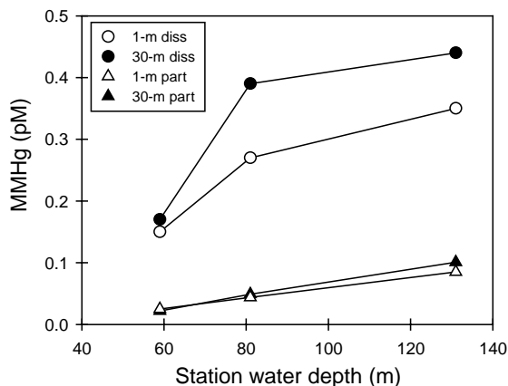
Fig. 11. Trends of increasing dissolved (diss; <0.2\text{-}\mu\text{m} filtered) and particle-associated (part; >0.2 \mu\text{m} ) MMHg with increasing water column depth in surface (1 m depth) and sub-thermocline (30 m) water on the continental shelf of southern New England.
