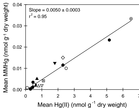
Fig. 4. Relation between reported average concentrations of MMHg and Hg(II) in surface sediments of different coastal marine systems. Hg(II) was presumed equal to total Hg for locations where Hg(II) was not reported; open circle (continental shelf of southern New England; this study); closed circles (South China, Bering, and Baltic Seas; Kannan and Falandysz, 1998); open square (Lagoon of Bizerte, Tunisia; Mzoughi et al., 2002); closed square (Patuxent River estuary, Maryland; Benoit et al., 1998); open triangle up (Bay of Biscay, France; Stoichev et al., 2004); closed triangle up (Long Island Sound, Connecticut/New York; Varekamp et al., 2000; Hammerschmidt and Fitzgerald, 2004); open dotted square (Gironde River estuary, France; Tseng et al., 2001); open triangle down (San Francisco Bay, California; Conaway et al., 2003); closed triangle down (Lavaca Bay, Texas; Bloom et al., 1999); open diamond (Chesapeake Bay, Maryland; Mason and Lawrence, 1999); closed diamond (Seine River estuary, France; Mikac et al., 1999); open hexagon (Saguenay Fjord, Quebec; Gagnon et al., 1997); closed hexagon (New York/New Jersey Harbor; Hammerschmidt, 2005); dotted open circle (estuarine section of Guanabara Bay, Brazil; Kehrig et al., 2003).
