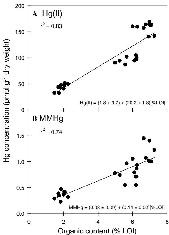
Fig. 2. Relation between the concentration of Hg species and organic content of surface sediments (upper 3 cm) on the continental shelf of southern New England.
