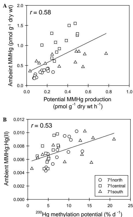
Fig. 8. Correlations between solid-phase MMHg and its potential gross rate of production in the upper 12 cm of sediment on the continental shelf of southern New England: (A) ambient MMHg concentration versus potential MMHg production estimated from ambient Hg(II) and incubations of added ^{200}\text{Hg} , and (B) solid-phase concentration ratio of ambient MMHg:Hg(II) versus ^{200}\text{Hg} methylation potential.
