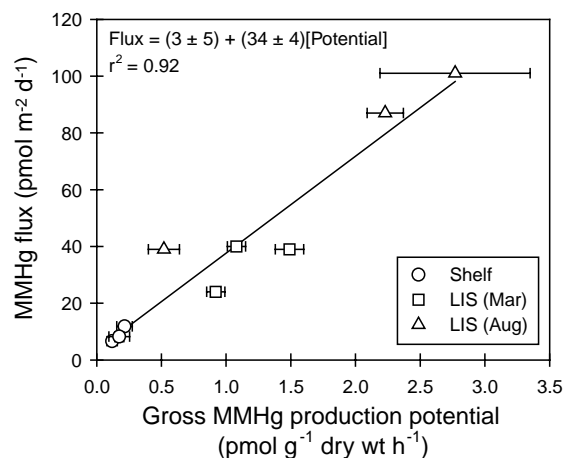
Fig. 9. Relation between estimated diffusive fluxes of dissolved MMHg ( <0.2\text{-}\mu\text{m} filtered) and gross potential rates of MMHg production in the upper 2 cm of sediment among sampling locations on the continental shelf and in Long Island Sound (LIS) in August 2001 and March 2002 (Hammerschmidt and Fitzgerald, 2004; Hammerschmidt et al., 2004). Error bars are \pm 1 SE of the mean. The uncertainty of LIS flux estimates was not determined. Data for LIS in June 2002 were not included because Hg methylation potentials were inhibited and MMHg fluxes enhanced by a seasonal change in sediment biogeochemistry following a spring plankton bloom.
