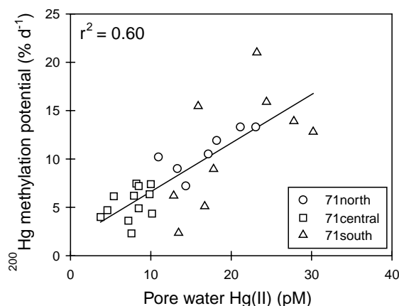
Fig. 6. Correlation between ^{200}\text{Hg} methylation potentials and levels of Hg(II) in filtered pore water of sediments on the continental shelf of southern New England.
