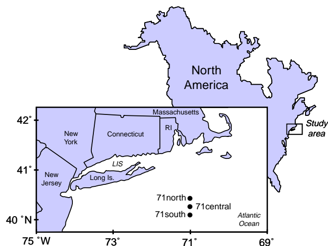
Fig. 1. Location of sediment sampling sites on the continental shelf of southern New England, northwestern Atlantic Ocean (71north, 40°44.20' N, 71°00.00' W; 71central, 40°28.00' N, 71°00.00' W; 71south, 40°12.00' N, 71°00.00' W).
