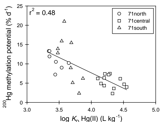
Fig. 7. ^{200}\text{Hg} methylation potential versus the distribution coefficient ( K_D ) of Hg(II) in sediments on the continental shelf of southern New England.
