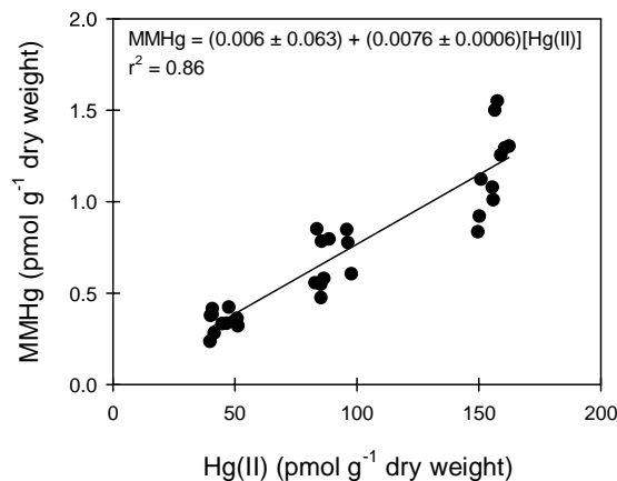
Fig. 3. MMHg versus Hg(II) in the upper 10 cm of sediment at three locations on the continental shelf of southern New England.
