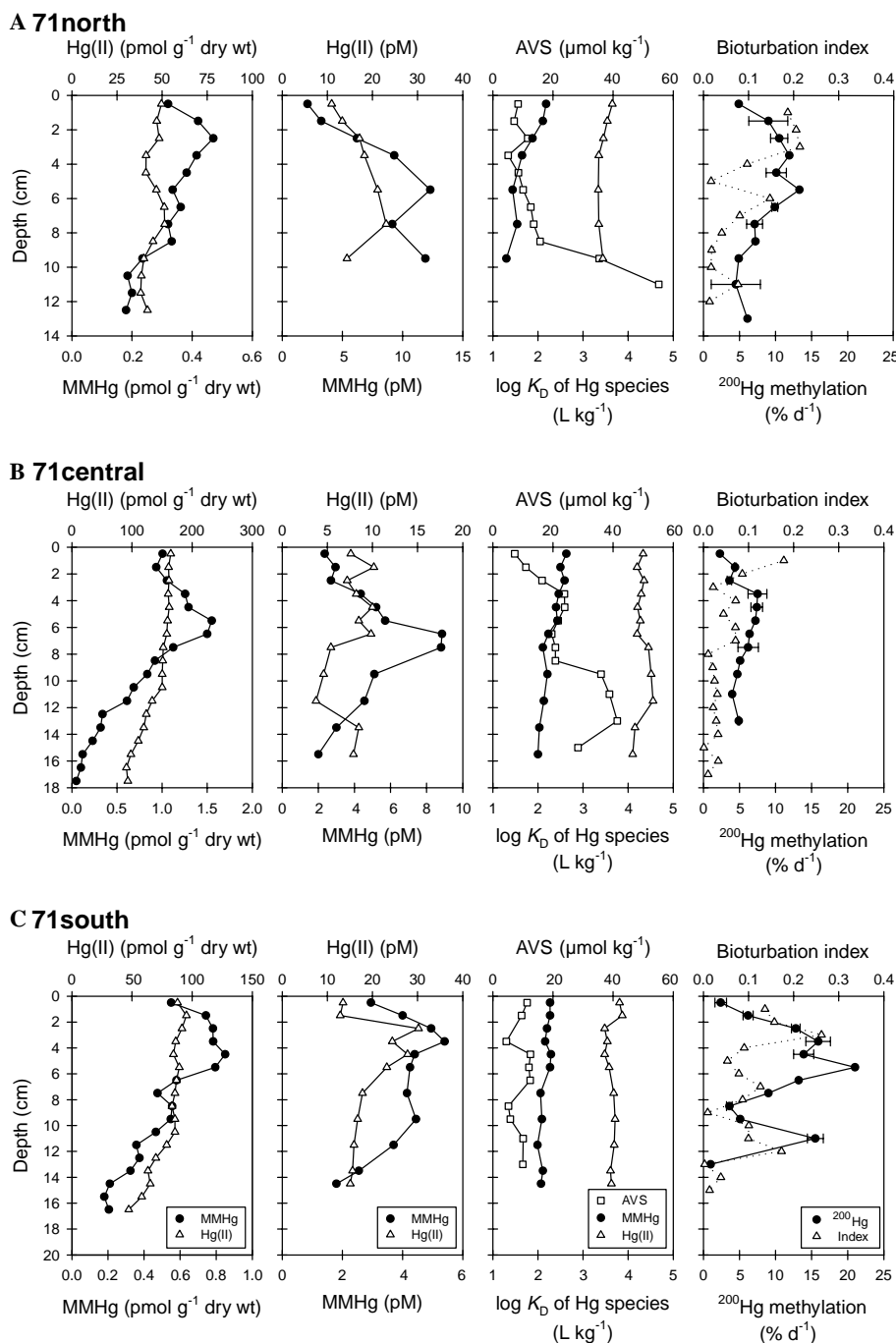
Fig. 10. Profiles of solid-phase and pore water Hg species, 200 Hg methylation potentials, and ancillary sediment biogeochemistry at three stations on the continental shelf of southern New England. Hg speciation profiles do not include results from the two surface sediment cores (upper 3 cm only) at each station. Error bars represent \pm 1 SE of the mean.
