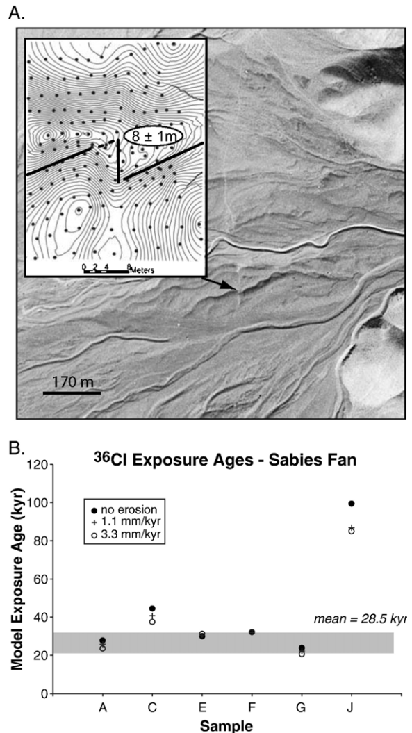
Fig. 6. Lateral displacement of boulder levee at Sabies Canyon (Site 4, Fig. 2). (A) Air photo of right-laterally displaced debris-flow levee on the Sabies Creek fan. Inset shows topographic map developed from differential GPS surveys (0.1 m contour interval, arbitrary datum). The levees are displaced by 8 \pm 1 m. (B) ^{36}\text{Cl} exposure ages for boulders at the Sabies Creek site. Ages are modeled for a range of weathering rates and mass loss from the boulder surface (0, 1.1, and 3.3 mm/ky). Two samples yielded anomalously old ages that are attributed to inheritance at the time of deposition. The range of ages for the remaining 4 samples suggest that the boulder levee was likely deposited between 22 and 32 ka. The absence of evidence for post-depositional erosion of the debris-flow surface suggests that the younger end of this range should most closely represent the age of the surface (see text for details).
