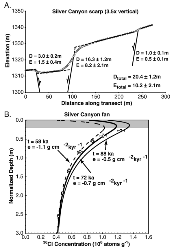
Fig. 5. Displacement across the White Mountain Fault Zone during Late Pleistocene time at Silver Canyon (Site 3, Fig. 2). (A) Topographic profile and reconstructed fault displacement based on projection of preserved fan surface and assumed fault dip. Uncertainties reflect a Monte Carlo propagation of uncertainty in fan slope, fault dip, and projection. We use estimates of net horizontal extension (E), with their associated uncertainties, to model the total fault slip on a single plane at depth (see text for details). (B) Fit of calculated ^{36}\text{Cl} concentration with depth to Silver Canyon (WAC01-01) normalized depth profile ^{36}\text{Cl} data. “ t ” is the exposure time, “ e ” is the surface erosion rate (negative values indicate profile aggradation). The “ t=72\text{ ka} ” curve is the best-fit profile and the “ t=88\text{ ka} ” and “ t=58\text{ ka} ” curves are the fits at the one-standard-deviation limits of the \Delta\chi^2 criterion (see appendix for details). Results suggest a depositional age of the fan surface of 72 \pm 15\text{ ka} .
