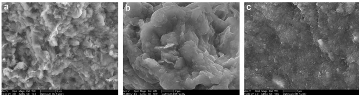
Figure 10. SEM images of soil matrices showing: (a) the flaky particle morphology of smectite in the Qt-5-1-B2 soil matrix; (b) the flaky smectite and spheroidal disordered kaolinite in the Qt-4-B2 soil matrix; and (c) the abundant spheroidal disordered kaolinite in the Qt-2-2-B2 bulk soil aggregate. Scale bars for a = 5 \mu\text{m} ; for b, c = 2 \mu\text{m} .
