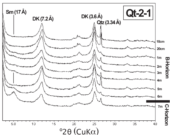
Figure 7. XRD data for the <2 \mu\text{m} fraction of EG-solvated powders from the 7 m Qt-2-1 (125 ka) terrace profile with delineated soil depths and B and C horizons.
