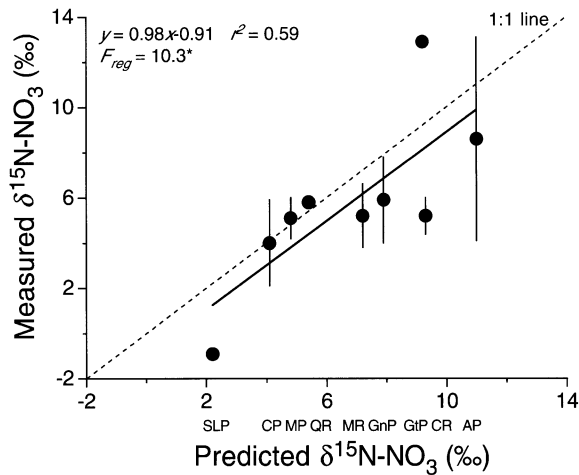
Figure 5. Predicted seepage face groundwater \delta^{15}\text{N-NO}_3 vs. measured groundwater \delta^{15}\text{N-NO}_3 for all nine watersheds. Dotted line is 1 to 1 line of perfect fit. Solid line is fit to data.
