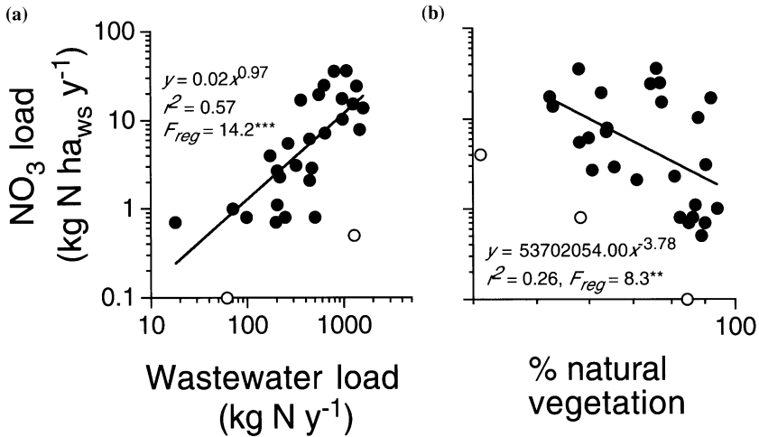
Figure 3. Mean NO 3 load to all nine receiving waters (kg N per hectare of watershed y -1 ) for each recharge zone vs. (a) recharge zone wastewater N load (kg N y -1 ) and (b) natural vegetation cover as a percent of total land area. *** = p < 0.001 , ** = p < 0.01 , * = p < 0.05 . Open circles are statistically determined outliers not included in regressions.
