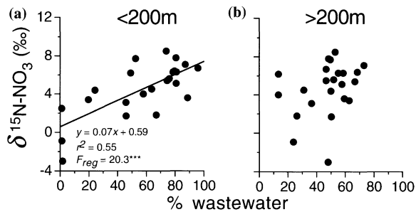
Figure 6. Mean \delta^{15}\text{N}\text{-NO}_3 for each recharge zone vs. recharge zone wastewater load as a percent of the total load. (a) data for the watershed within 200 m of shore, and (b) data for the watershed greater than 200 m from shore.
