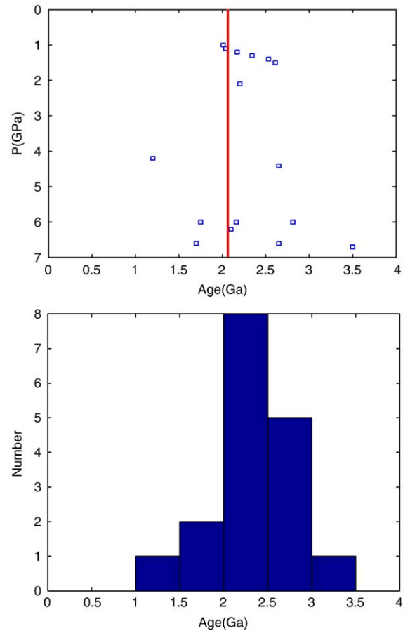
Fig. 3. Rhenium-depletion minimum ages of xenoliths as a function of pressure (top), as well as histogram of Premier ages (bottom). Red line corresponds to age of Bushveld (2.06 Ga). Most xenoliths predate the Bushveld intrusion, and there is no evidence of younging with depth as predicted by delamination hypothesis (data from [41]). Pressures in spinel stability field (less than 2 GPa) are nominal values. Sheared nodules have no pressure estimate but are assumed to be deep and placed arbitrarily at 6 GPa.
