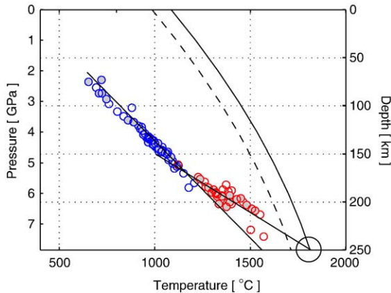
Fig. 4. P - T estimates obtained from mantle xenoliths taken from the Archean Kaapvaal craton and adjacent areas [57]. Blue circles represent low temperature xenoliths; red circles show high temperature xenolith data. Pressures are calculated after Finnerty and Boyd [83], and temperatures are calculated using both the O'Neill and Wood [84] (open symbols) and MacGregor [85] (filled symbols) methods. Straight lines show best-fit regression lines through the low and high temperature data. The regression through the high temperature xenolith data predicts a mantle temperature of \sim 1850 °C at the base of the lithosphere. Curved lines represent estimates of depleted-mantle solidus (solid line) [86] and fertile-mantle (dashed) solidus assumed to be 100 °C less, based on the systematics of the MELTS algorithm [52]. Note that extrapolated geotherm from high temperature xenoliths crosses the fertile-mantle solidus at about 235 km depth.
