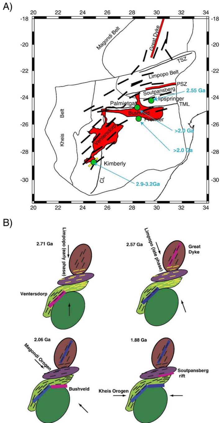
Fig. 2. (A) Map of southern Africa showing major rift systems with basaltic magmatism: Great Dyke, Venterdorp (surface exposures shown), Bushveld, and Soutpansberg. Also shown, shear-wave splitting fast polarization directions (from [82]). Abbreviations: TML: Thabazimbi Murchison Lineament, CL: Colesberg Lineament, PSZ, Palala Shear Zone, TSZ, Triangle shear zone. Green filled circles denote locations of kimberlite pipes, whose mantle xenoliths sample the mantle beneath the Venterdorp and Bushveld. Ages of nodules are denoted in blue. (B) Schematic illustrating development of collisional rifts and basaltic magmatism in southern Africa. Arrows show compression direction of orogen. Short lines show mantle fabric inferred from seismic anisotropy, which is either being formed (yellow) or fossilized (black). Red (blue) bars denote magmatic events during (after) activity. Top-left: Emplacement of the Venterdorp supergroup due to the early phase of the Limpopo orogen (2.71 Ga). Top-right: Emplacement of the Great Dyke due to the late phase of the Limpopo orogen (2.57 Ga). Bottom-left: Reactivation of Limpopo structures by Magondi Orogen and the creation of a collisional rift that produced the Bushveld Intrusion (2.06 Ga). Bottom-right: Creation of the collisional Soutpansberg Rift by the Kheis Orogen (1.88 Ga). After Silver et al. [15].
