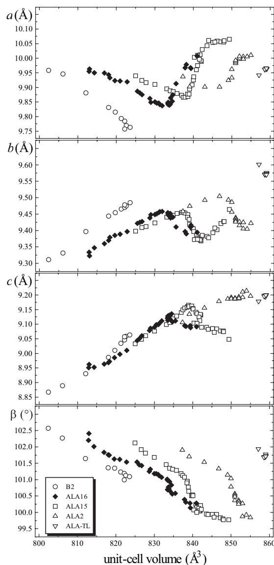
FIGURE 2. The a , b , c (Å), and \beta (°) parameters vs. the unit-cell volumes (Å 3 ).
