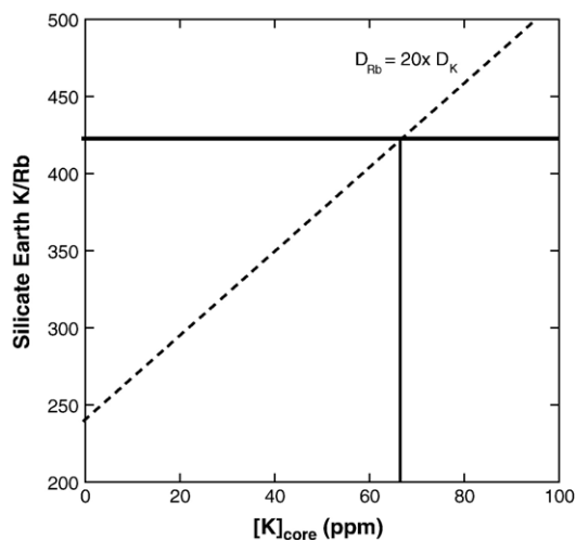
Fig. 5. Correlation of core K content and K/Rb in the residual Silicate Earth, assuming batch metal/silicate segregation, and a high- P metal/silicate D_{\text{Rb}}=20 \times D_{\text{K}} [61]. For an estimated K/Rb of \sim 420 for the Silicate Earth [34], core K content is limited to less than \sim 60 ppm, assuming a starting Bulk Earth composition similar to CI chondrites. For a Silicate Earth K content of 150 ppm [28], the resultant Rb/Sr ratio of \sim 250 would limit the amount of K in the core to less than 10 ppm.
