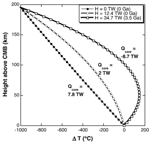
Fig. 3. Equilibrium thermal profile for a 200 km thick conductive boundary layer at the base of the mantle with variable internal heat production. Temperature contrast between the top and bottom of the layer is fixed at 1000 °C, at the low end of estimates for core/mantle temperature contrast. Temperature profiles are calculated assuming dT/dr \neq 0 at every depth, so that for a given thin shell with radius r , Q_{r, out} = Q_{r, in} + H_r ; Q_r denotes heat flow into and out of the shell and H_r the rate of internal heat production within the shell.
