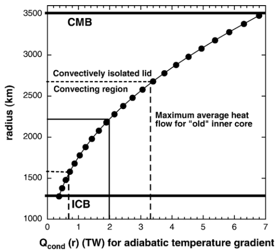
Fig. 2. Conductive heat flow along an adiabatic temperature gradient in the outer core. The adiabatic temperature gradient and thermal conductivity are assumed to vary smoothly between the outer and inner core boundaries, from 0.97 \text{ K km}^{-1} to 0.27 \text{ K km}^{-1} and from 46 to 63 \text{ W K}^{-1} \text{ m}^{-1} , respectively [22,65,66]. Solid and dashed horizontal lines indicate the approximate thickness of an upper outer core hot thermal layer for a reduced core/mantle heat flow of 2 \pm 1.3 \text{ TW} . Q_{\text{cond}}(r) of 3.3 \text{ TW} (the upper limit for an “old” inner core) requires an \sim 800 \text{ km} thick upper thermal boundary layer. Reduction in the estimated thermal conductivity (e.g., to reduce estimated Q_{\text{cond}}(3480) from 7 to 5 \text{ TW} ) will reduce the minimum thickness of the hot upper boundary layer from \sim 800 \text{ km} to \sim 500 \text{ km} . See text for details.
