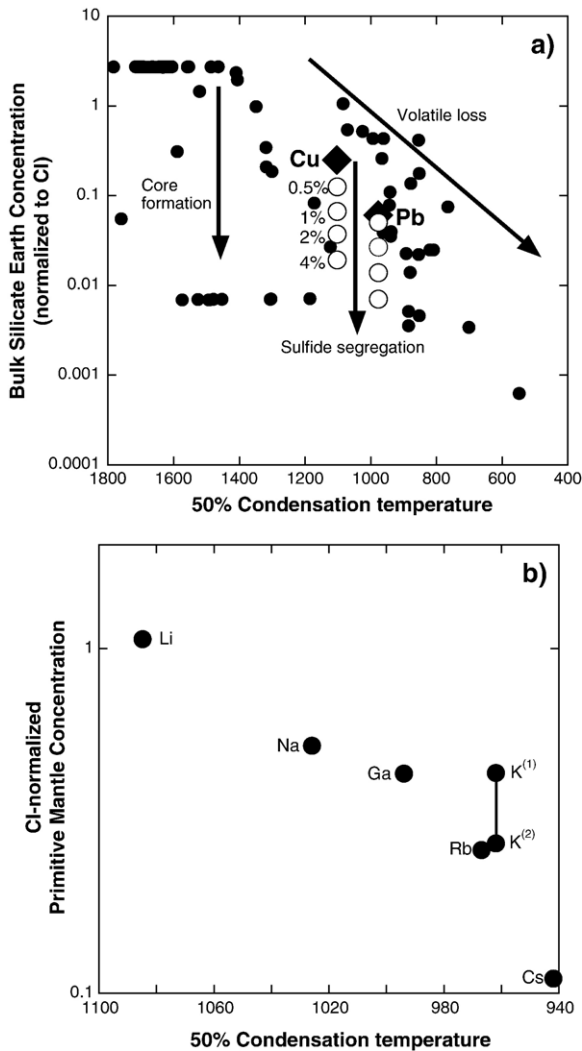
Fig. 4. (a) CI-normalized elemental abundances in the Silicate Earth [34] versus 50% condensation temperature at 10^{-4} atm [58]. Most lithophile elements display a strong correlation between normalized abundance and condensation temperature, reflecting partial volatile loss of non-refractory elements either prior to or during Earth accretion. Departures from the volatile depletion trend primarily reflect core segregation of siderophile or chalcophile elements. The effect of sulfide segregation on Cu and Pb abundances is shown (open circles), assuming sulfide/silicate D_{Cu} and D_{Pb} \approx 500 and 1000, respectively [10,53]. Cu and Pb abundances estimated for the Silicate Earth are consistent with <0.5\% sulfide segregation during core formation. (b) Elemental abundance versus condensation temperature for the alkali metals and gallium. Two estimates of K relative abundance range from 240 ppm (1: [34]) to 150 ppm (2: [28]). The alkali metals show a smooth trend of increasing depletion in the Silicate Earth with decreasing condensation temperature, particularly if the lower K abundance estimate of [28] is considered.
