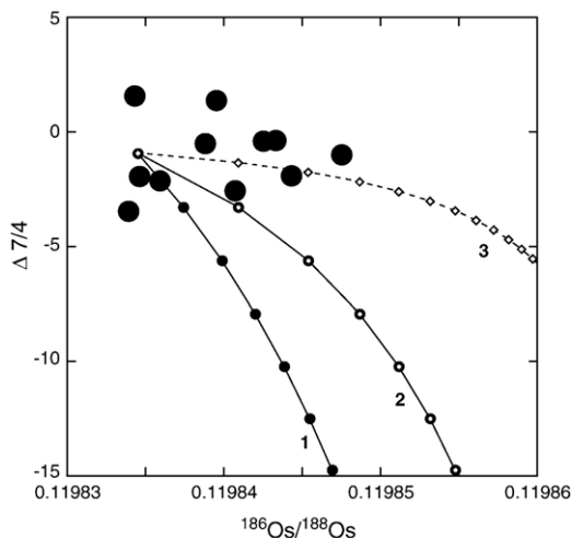
Fig. 1. Os- and Pb-isotope variations in Hawaiian picrites. \Delta 7/4 = 100 * ((^{207}\text{Pb}/^{204}\text{Pb})_{\text{measured}} - ^{207}\text{Pb}/^{204}\text{Pb}_{\text{NHRL}}) , where ^{207}\text{Pb}/^{204}\text{Pb}_{\text{NHRL}} = Northern Hemisphere Reference Line ^{207}\text{Pb}/^{204}\text{Pb} calculated for the measured ^{206}\text{Pb}/^{204}\text{Pb} [13]. Hawaiian data are from [2] and references therein. The effects of core addition are shown for three core composition models. Tick marks represent 0.1% core addition to primitive mantle [34]. Core ^{186}\text{Os}/^{188}\text{Os} is from [3]. Core Pb-isotope composition is assumed to resemble Canyon Diablo troilite [64]. See text for other mixing parameters.
