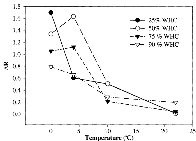
Figure 4. The relative effect of post-fire changes in respiration that could not be explained by either temperature or moisture ( \Delta R ). \Delta R was estimated as the ratio of the difference in \text{CO}_2 emissions between burned and control samples to emissions from control samples.
