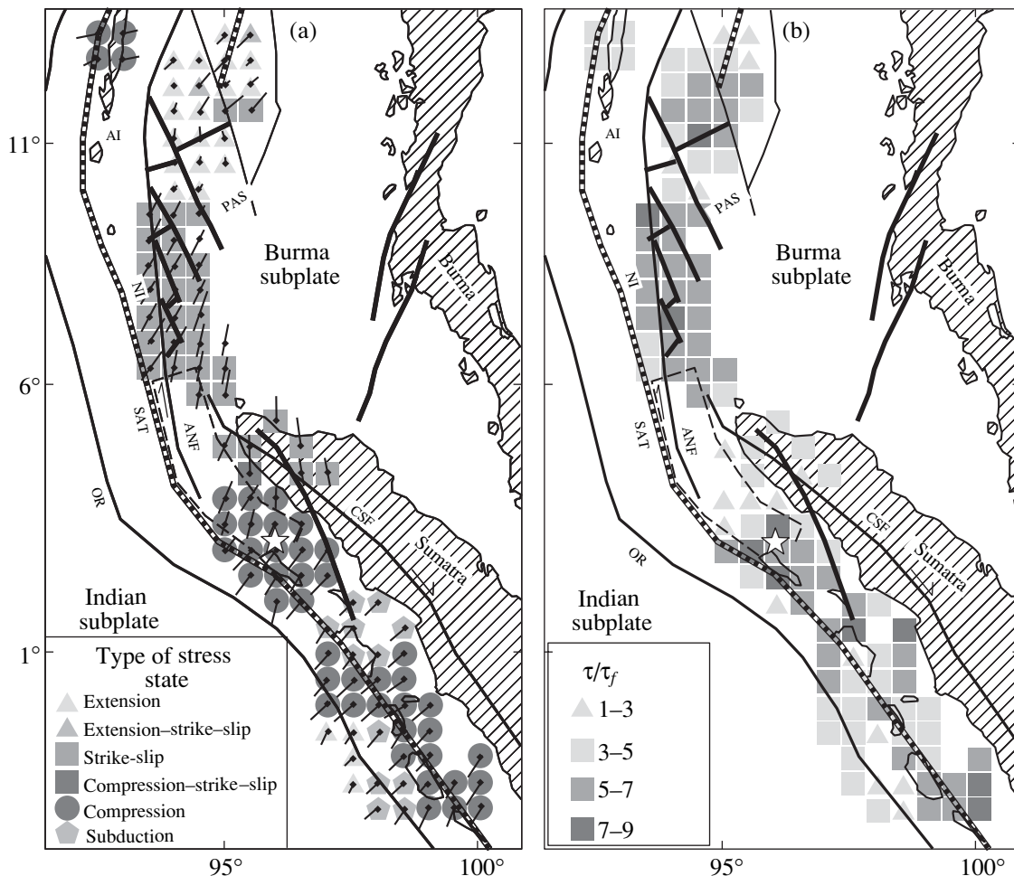
Fig. 1. Results of reconstruction natural stresses: (a) orientation of horizontal plane projections of subsidence axes of maximum compression stresses \sigma_3 and type of stressed state; (b) relative values of maximum tangential stress (normalized to internal cohesion of rock massifs). An asterisk indicates the beginning of SAE initiation; dashed segment is the SAE source region near the northern boundary of Sumatra [5]. (CSF) Central Sumatra Fracture; (ANF) Andaman-Nicobar Fracture; (SAT) Sunda-Andaman Trough; (OR) oceanic ridge; (PAS) pull-apart back-arc structures; (AI) Andaman Islands; (NI) Nicobar Islands.
