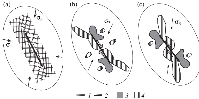
Fig. 2. Results of theoretical solution of the strike-slip fracture problem [Osokina, 1987]. (a) Orientation of the axes of principal stresses: (1) \sigma_1 , (2) \sigma_3 ; (b) regions of (3) decrease and (4) increase in maximum tangential stresses relative to the regional state (observed before the activation of the fracture) for values of the angle between the axis of maximum regional compression and fracture plane equal to (b) 30^\circ and (c) 60^\circ .
