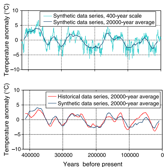
Fig. 16. (Up) Plot of the synthetic time series generated by the toy model fitted to the adapted Vostok data set; (down) comparison of the synthetic and original time series in terms of their 20,000-year moving averages.
