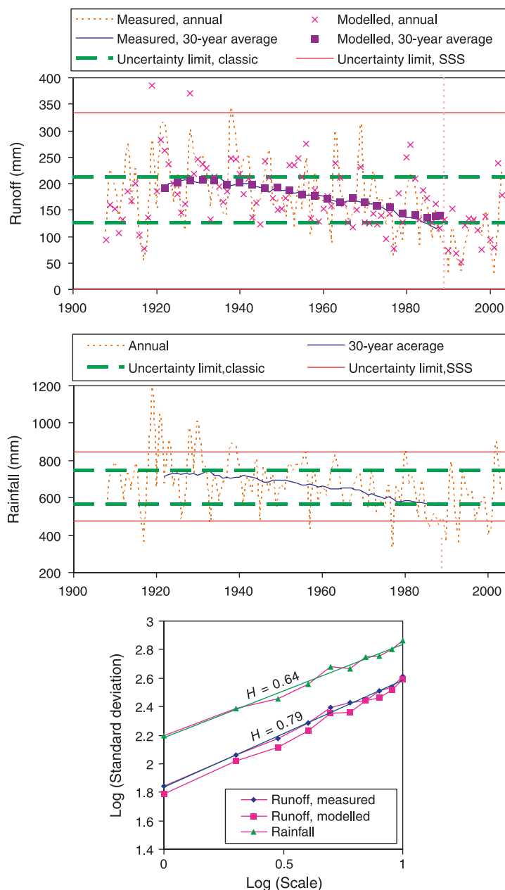
Fig. 1. (Up) Plot of the Boeotikos Kephisos river runoff series, both measured and modelled, in annual and 30-year timescales, and of the 95% confidence limits for the 30-year scale, estimated by Monte Carlo simulation. (Middle) Plot of the rainfall series at the same catchment in annual and 30-year timescales, and of the corresponding 95% confidence limits for the 30-year scale. (Down) Aggregated standard deviation plot of the series.
