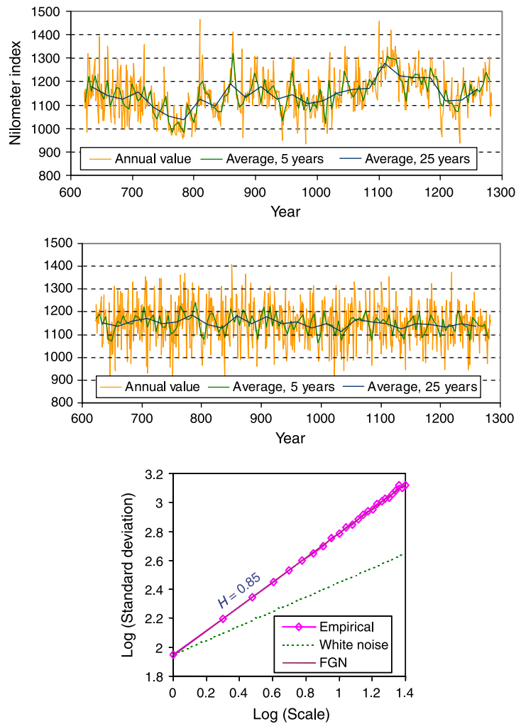
Fig. 2. (Up) Plot of the Nilometer series indicating the annual minimum water level of the Nile River for the years 622–1284 AD (663 years); (middle) a synthetic white noise series, for comparison; (down) aggregated standard deviation plot of the series.
