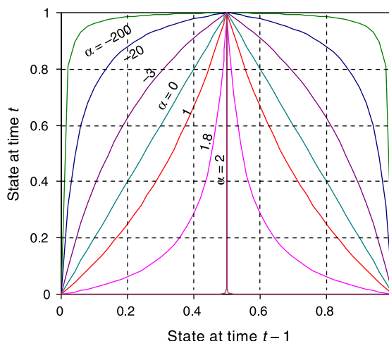
Fig. 9. The generalised tent map for different values of its parameter \alpha .
