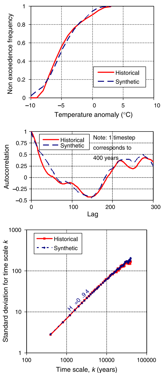
Fig. 19. Comparison of statistical properties of the original Vostok time series and the synthetic one of Fig. 18: (up) distribution function; (middle) autocorrelogram; (down) aggregated standard deviation plot.
