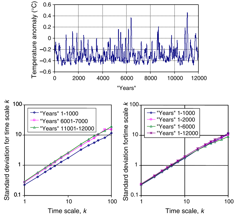
Fig. 22. (Up) Plot of the 50-year moving average of the synthetic time series of Fig. 14, corresponding to the Jones data set, but extended to the length 12,000 ‘years’; (down) aggregated standard deviation plots of several parts of the 12,000-year series.
