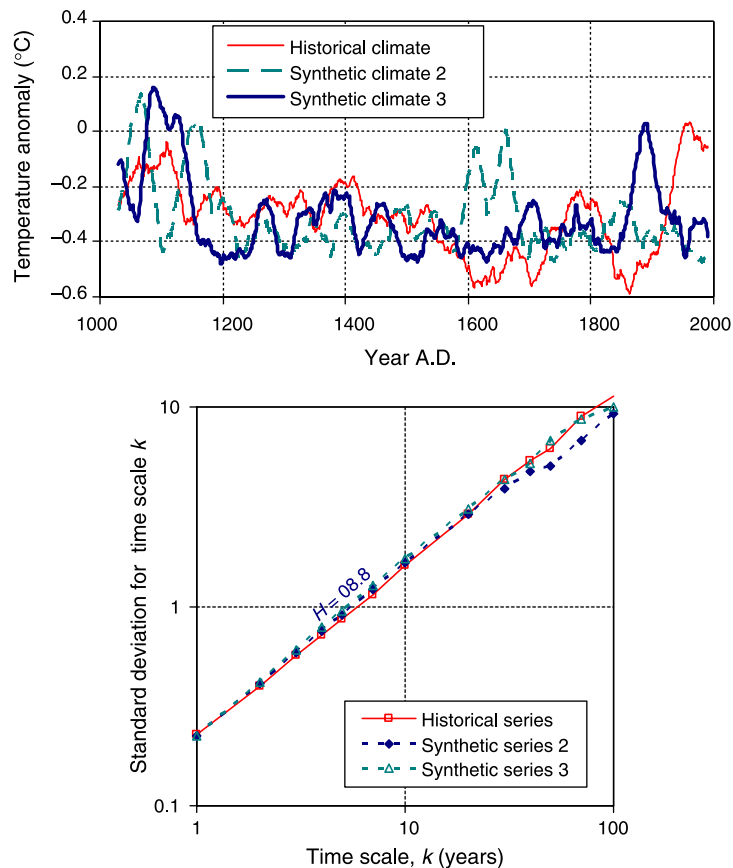
Fig. 21. (Up) Comparison of the synthetic series 2 and 3 of Fig. 20, and the original Jones series in terms of their moving averages of the past 30 years for all the 1000-year period; (down) comparison of the aggregated standard deviation plots of the three series.
