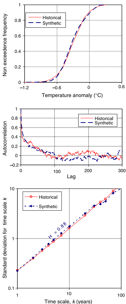
Fig. 15. Comparison of statistical properties of the original Jones time series and the synthetic one of Fig. 14: (up) distribution function; (middle) autocorrelogram; (down) aggregated standard deviation plot.
