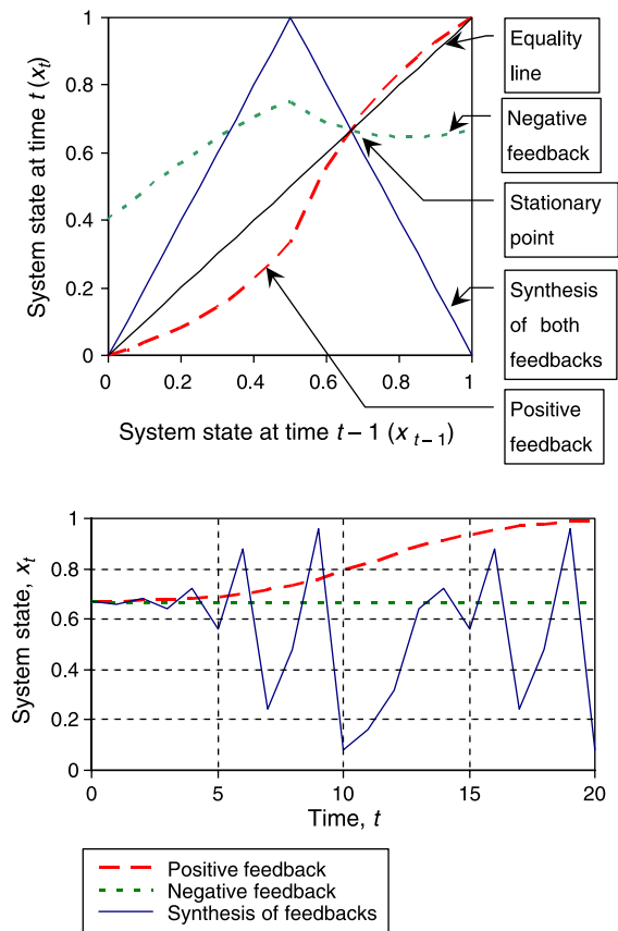
Fig. 8. (Up) Schematic of the dynamics of a system subject to a feedback loop with a positive and a negative reaction; (down) evolution of the system under the positive, negative or both reactions, when it starts from very close to its fixed point ( x^*=2/3 , x_0=0.67 ).
