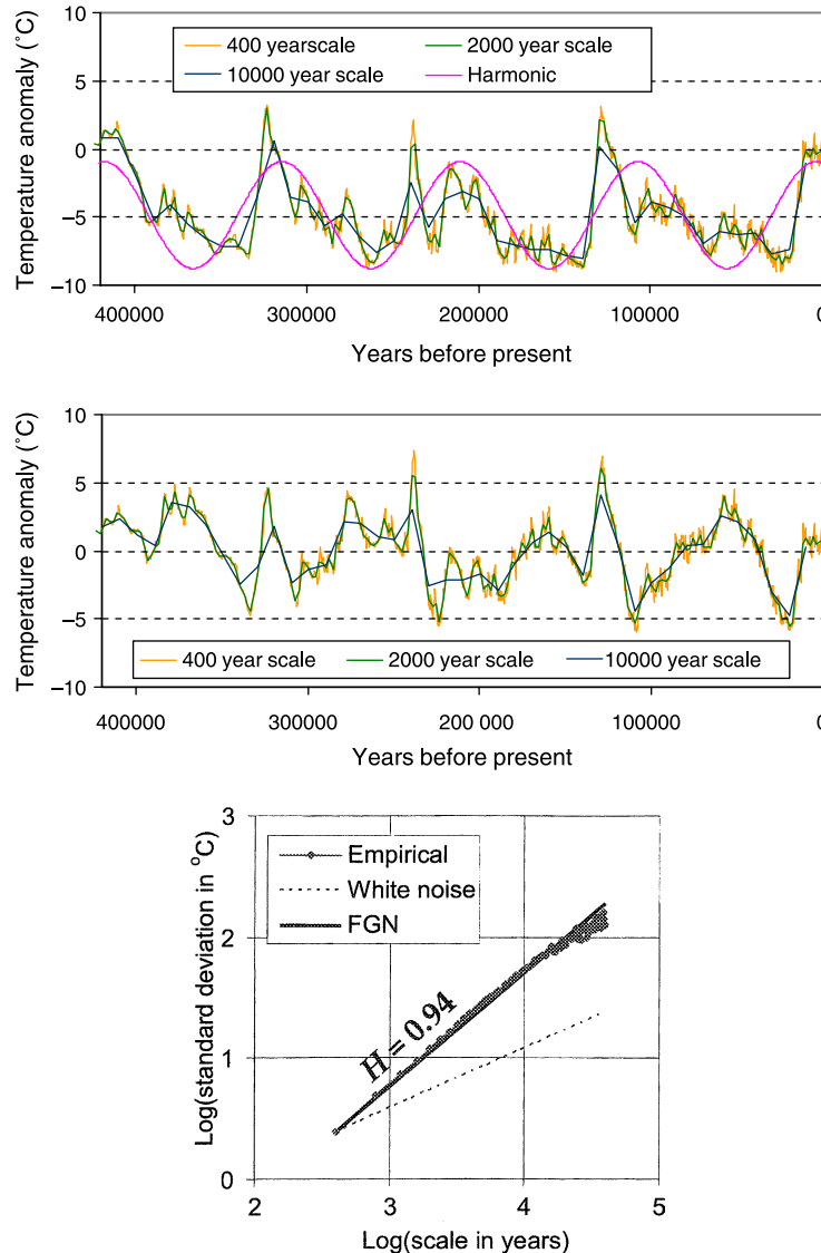
Fig. 6. (Up) Fitting of the principal harmonic for the temperature difference of the Vostok data set; (middle) plot of the adapted, by subtraction of the principal harmonic, temperature difference of the Vostok data set; (down) aggregated standard deviation plot of the adapted series.
