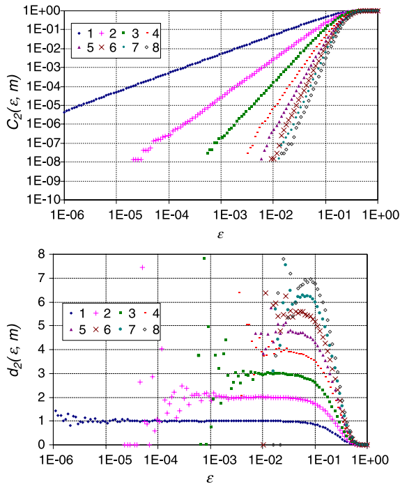
Fig. 23. Plots of the correlation sums C_2(\epsilon, m) (up) and their local slopes d_2(\epsilon, m) (down) versus the scale length \epsilon for embedding dimension m=1 to 8, for the 12,000-year synthetic time series of Fig. 22 corresponding to the Jones data set.
