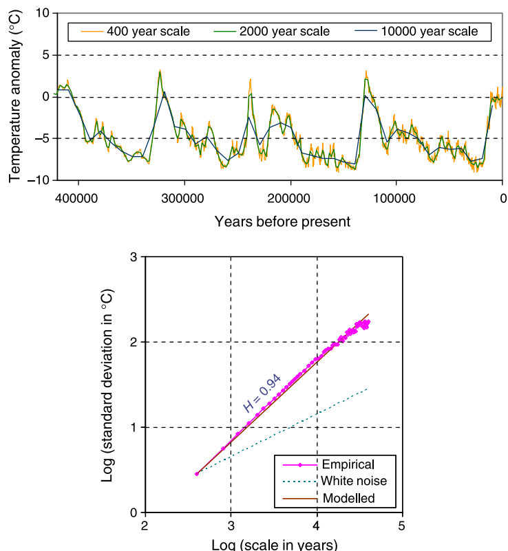
Fig. 4. (Up) Plot of the temperature difference, with reference to the mean recent time value, from the Vostok ice core deuterium data set going back to 422,766 years before present; (down) aggregated standard deviation plot of the series.
