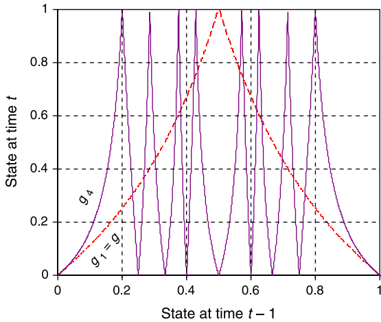
Fig. 10. Synthesis of four generalised tent maps for \alpha=1 .
