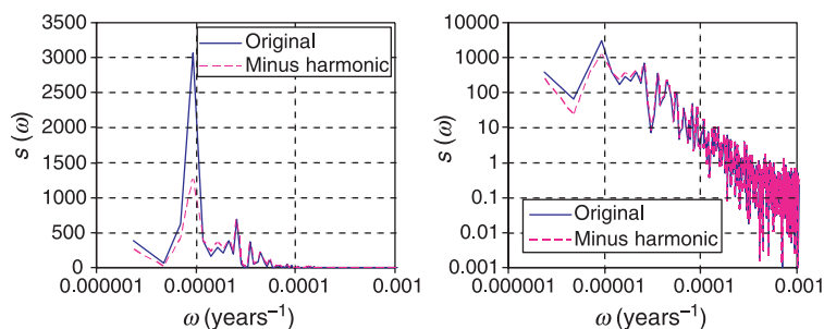
Fig. 5. Periodogram of the Vostok temperature time series in Cartesian (left) and logarithmic (right) ordinates.
