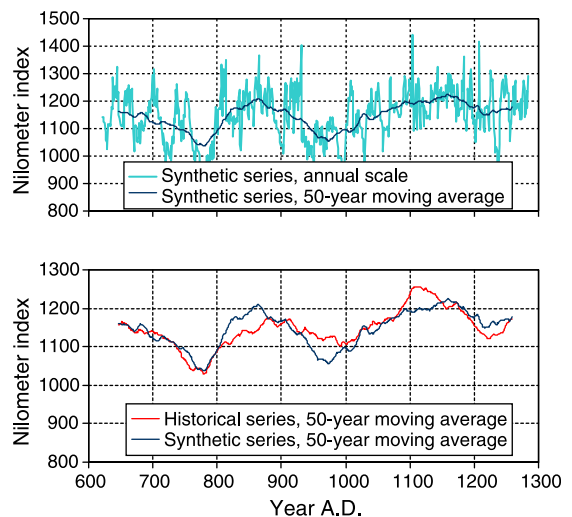
Fig. 12. (Up) Plot of the synthetic time series generated by the toy model fitted to the Nilometer data set; (down) comparison of the synthetic and original time series in terms of their 50-year moving averages.
