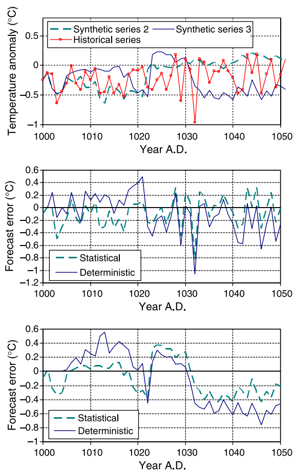
Fig. 20. (Up) Plot of the first 50 years of evolution of the historical Jones data series and two synthetic time series (synthetic series 2 and 3), similar to that of Fig. 14 (synthetic series 1) but with initial values u_0 and \alpha_0 estimated so that the synthetic series match the historical one at the first two values with the only difference between series 2 and 3 being that the initial value \alpha_0 in the latter is greater by 0.00001% than in the former; (middle) comparison of forecast errors of two forecast methods, (a) statistical, in which the forecast is the average of synthetic series 2 for the 50-year period, and deterministic, in which the forecast is the synthetic series 2; (down) same as in the middle panel but assuming that the actual evolution is that of synthetic series 3.
