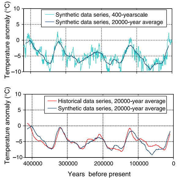
Fig. 18. (Up) Plot of the synthetic time series of Fig. 16 to which the harmonic with period 103,598 years has been added; (down) comparison of this series with the original Vostok data series in terms of their 20,000-year moving averages.
