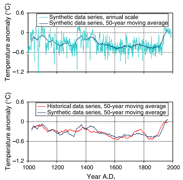
Fig. 14. (Up) Plot of the synthetic time series generated by the toy model fitted to the Jones data set; (down) comparison of the synthetic and original time series in terms of their 50-year moving averages.
