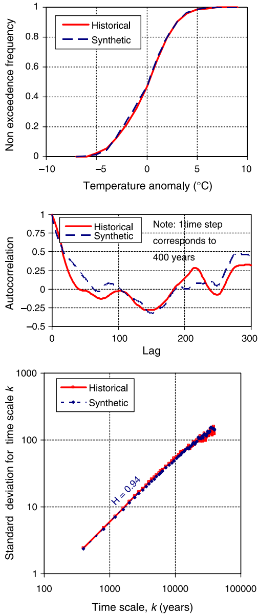
Fig. 17. Comparison of statistical properties of the adapted Vostok time series and the synthetic one of Fig. 16: (up) distribution function; (middle) autocorrelogram; (down) aggregated standard deviation plot.
