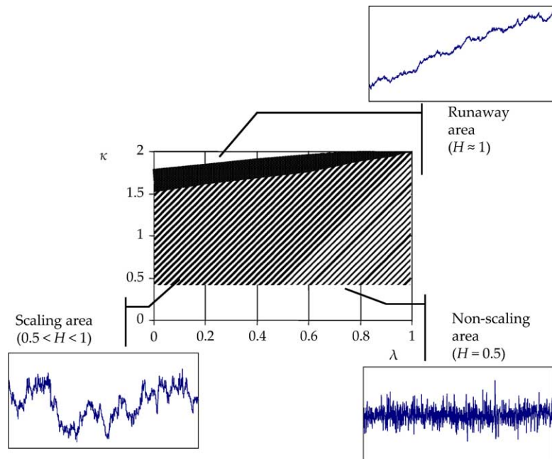
Fig. 11. Schematic of the general behaviour of the double tent map in terms of the ranges of its parameters \kappa and \lambda . The shaded area corresponds to n=1 and the dark area to n=4 .
