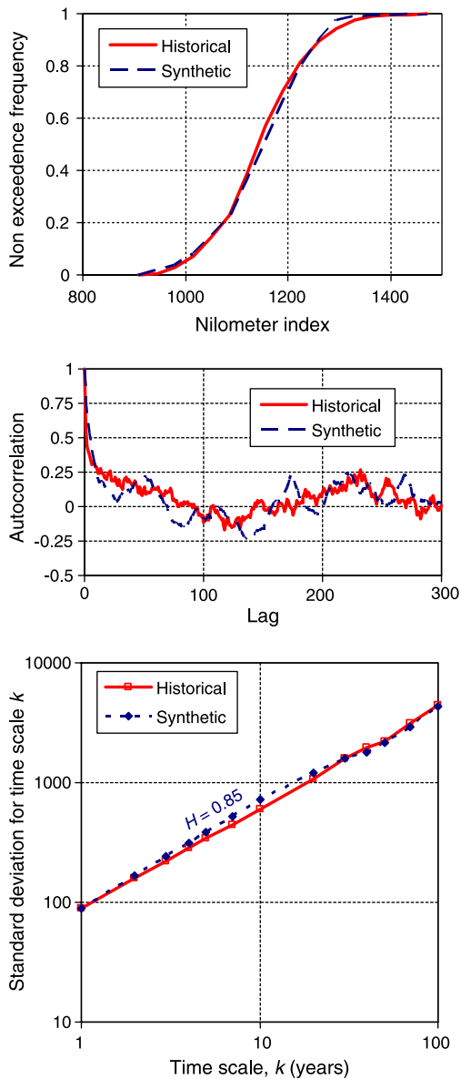
Fig. 13. Comparison of statistical properties of the original Nilometer time series and the synthetic one of Fig. 12: (up) distribution function; (middle) autocorrelogram; (down) aggregated standard deviation plot.
