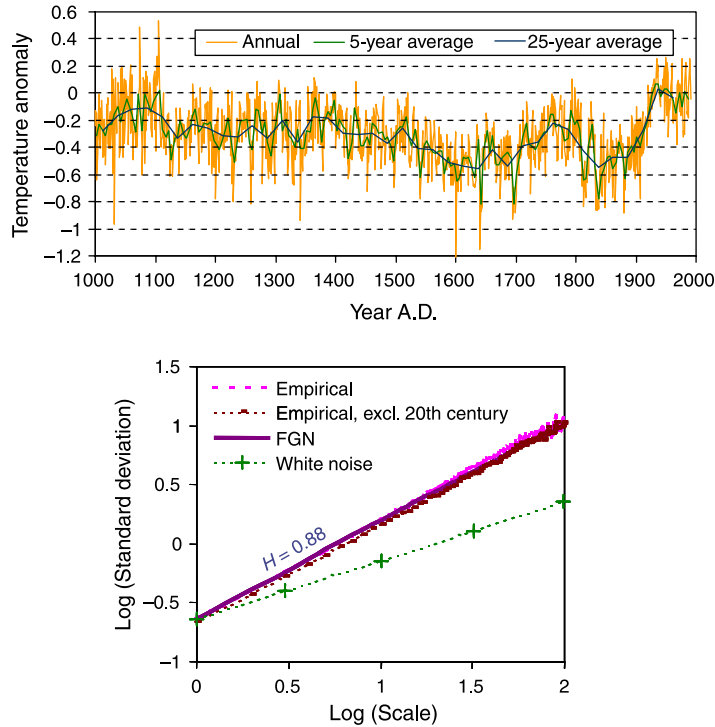
Fig. 3. (Up) Plot of the Northern Hemisphere temperature anomalies in °C with reference to 1961–1990 mean (992 years, Jones data set); (down) aggregated standard deviation plot of the series.
