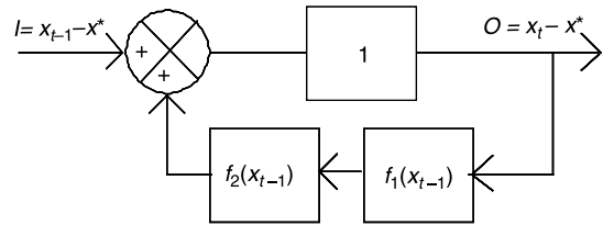
Fig. 7. Schematic of a simplified representation of a climatic system with a feedback loop including a positive and a negative reaction.
